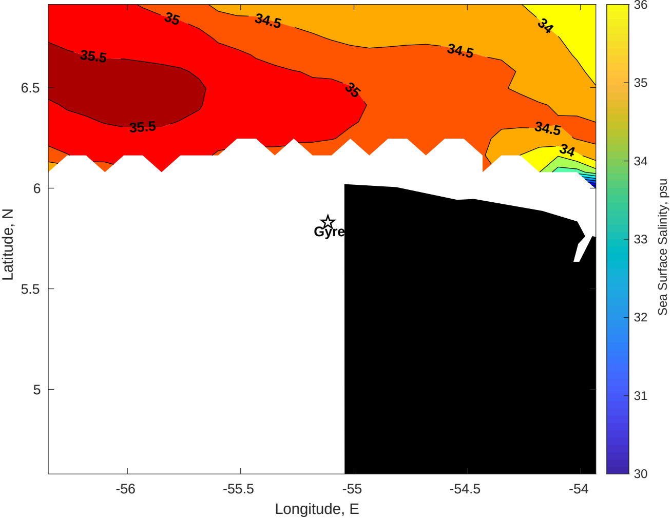
Surface Salinity for Gyre at 15-Aug-2025 00:00:00
