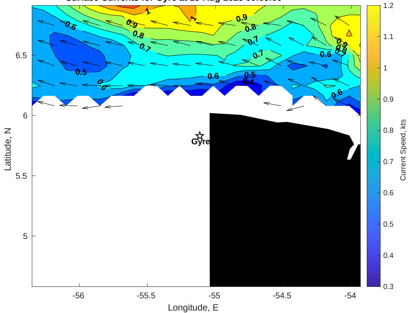
Surface Currents for Gyre at 15-Aug-2025 00:00:00
