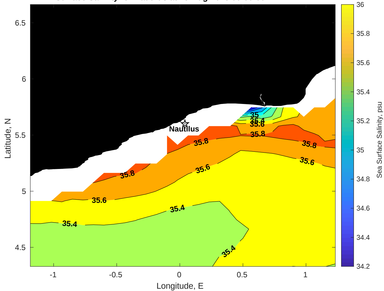
Surface Salinity for Nautilus at 15-Aug-2025 00:00:00
