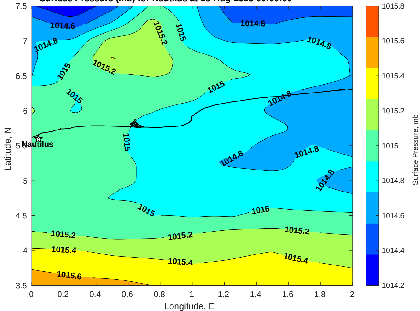
Surface Pressure (mb) for Nautilus at 18-Aug-2025 00:00:00
