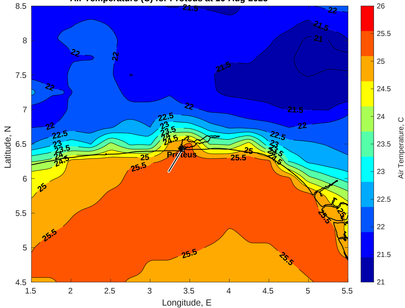
Air Temperature (C) for Proteus at 16-Aug-2025
