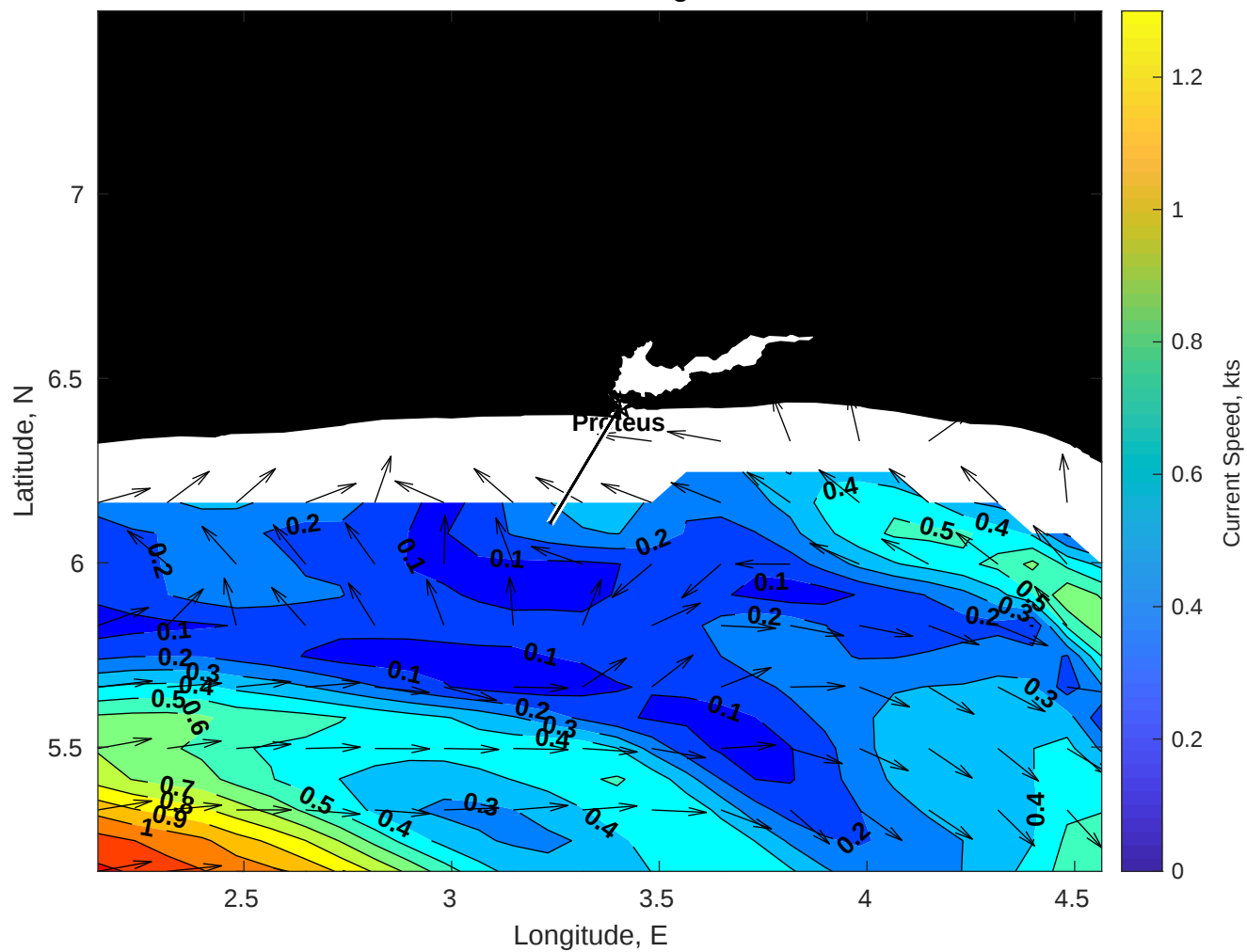
Surface Currents for Proteus at 15-Aug-2025 00:00:00
