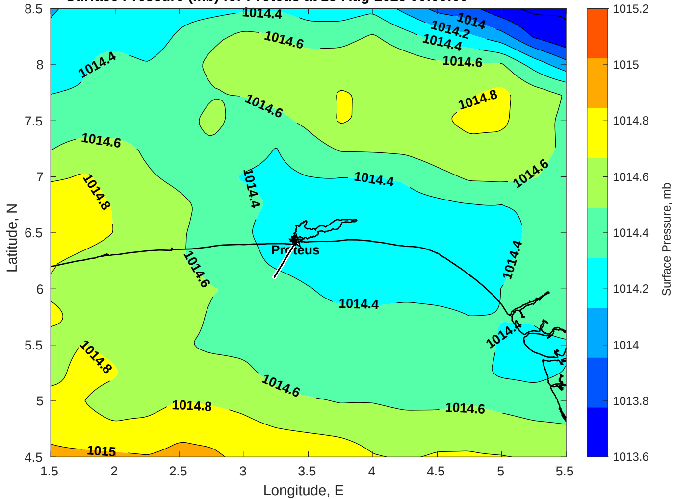
Surface Pressure (mb) for Proteus at 18-Aug-2025 00:00:00
