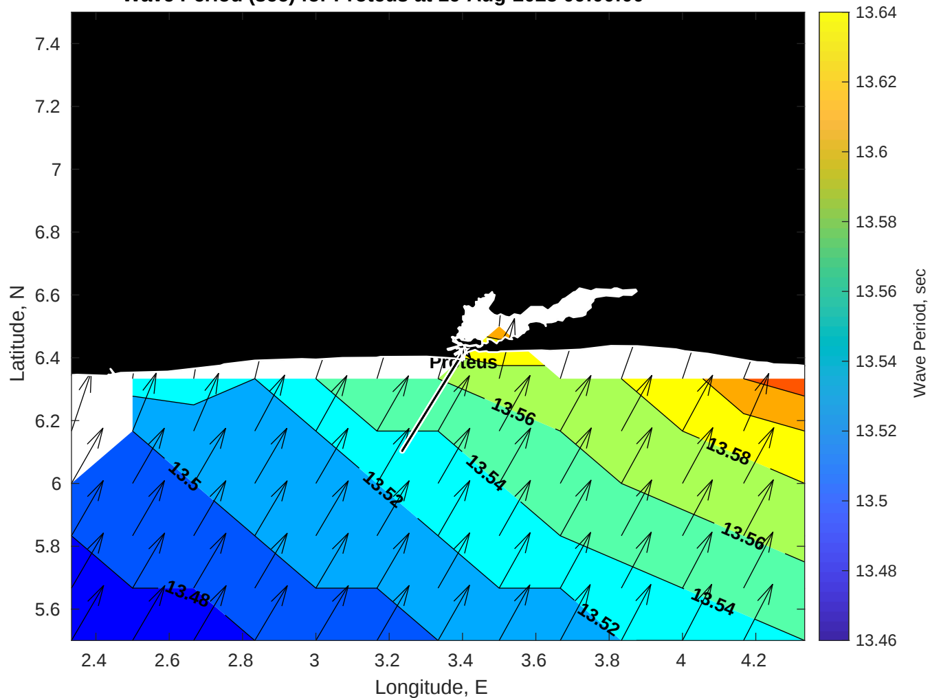
Wave Period (sec) for Proteus at 16-Aug-2025 09:00:00
