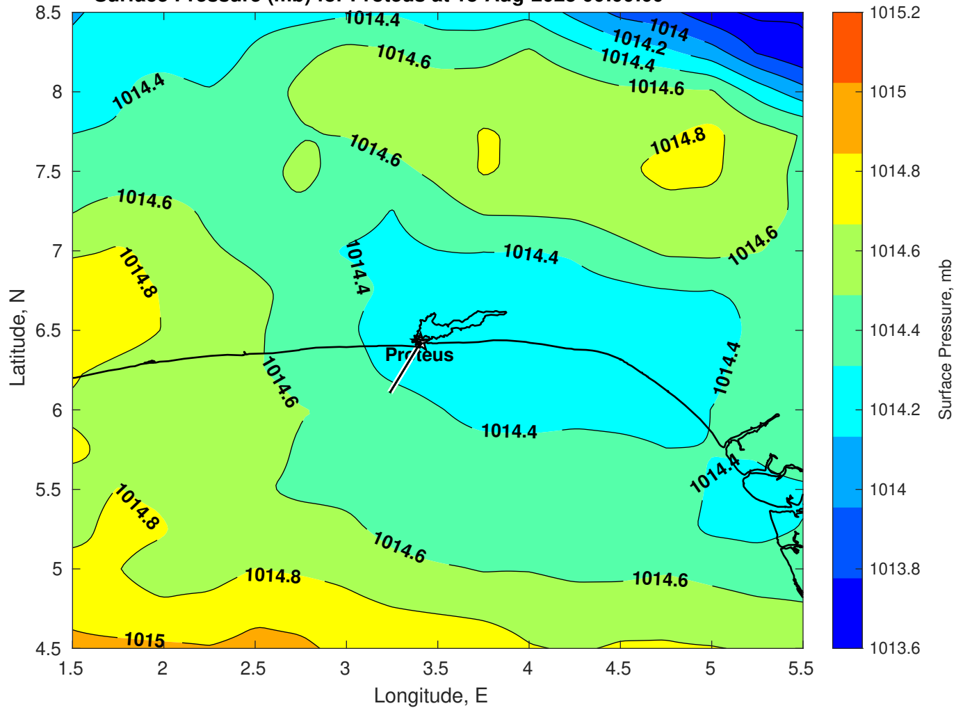
Surface Pressure (mb) for Proteus at 18-Aug-2025 00:00:00
