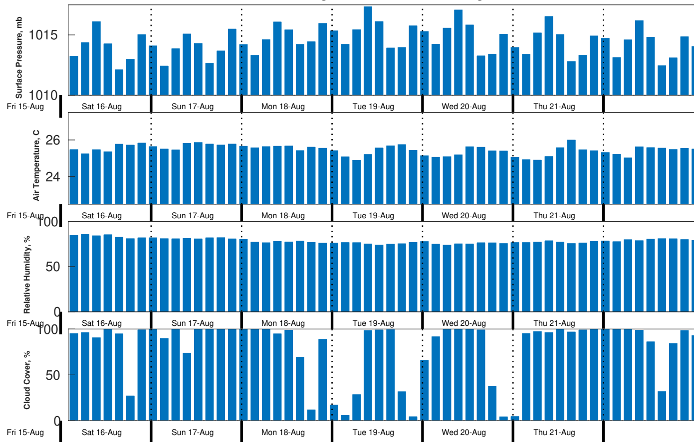
Met Forecast for Proteus from 16-Aug-2025 00:00:00 to 23-Aug-2025 00:00:00
