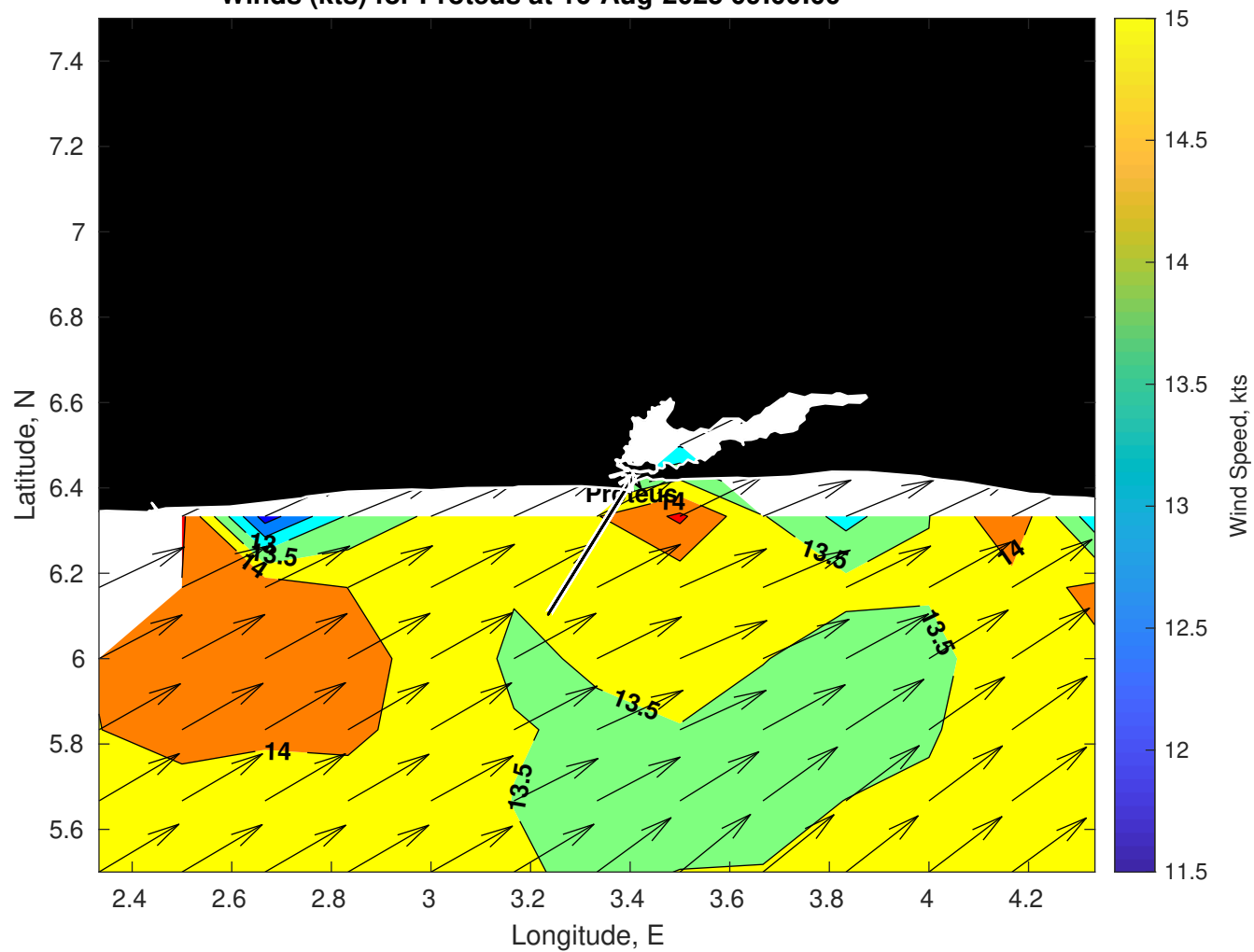
Winds (kts) for Proteus at 16-Aug-2025 09:00:00
