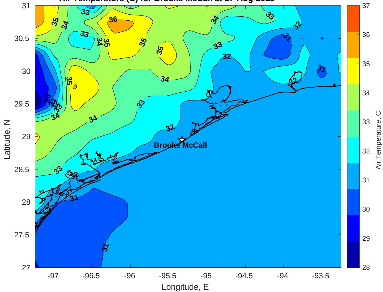
Air Temperature (C) for Brooks McCall at 17-Aug-2025
