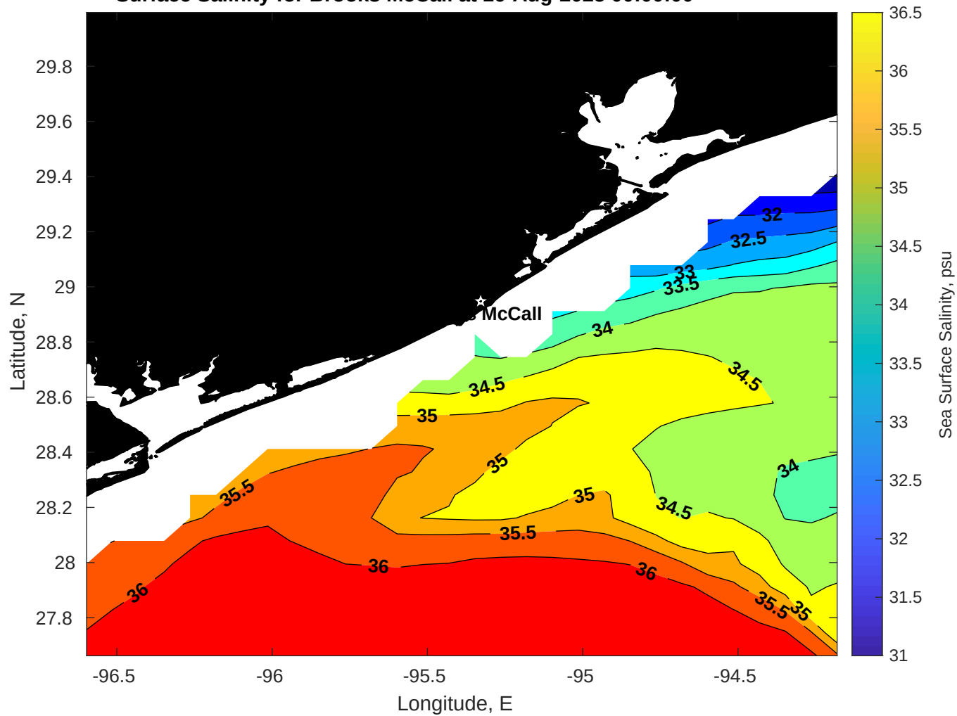
Surface Salinity for Brooks McCall at 16-Aug-2025 00:00:00
