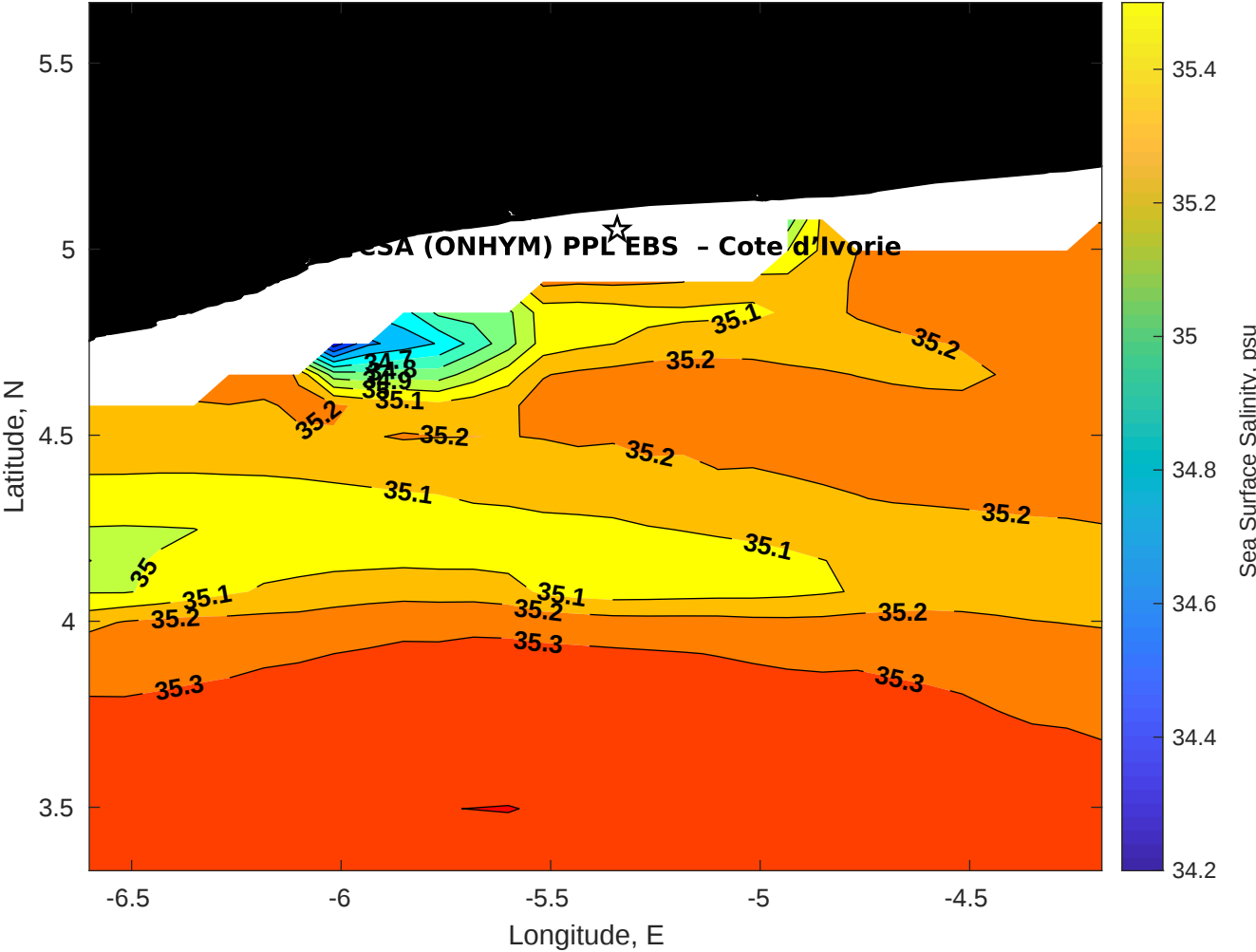
Surface Salinity for CSA (ONHYM) PPL EBS - Cote d'Ivoire at 16-Aug-2025 00:00:00
