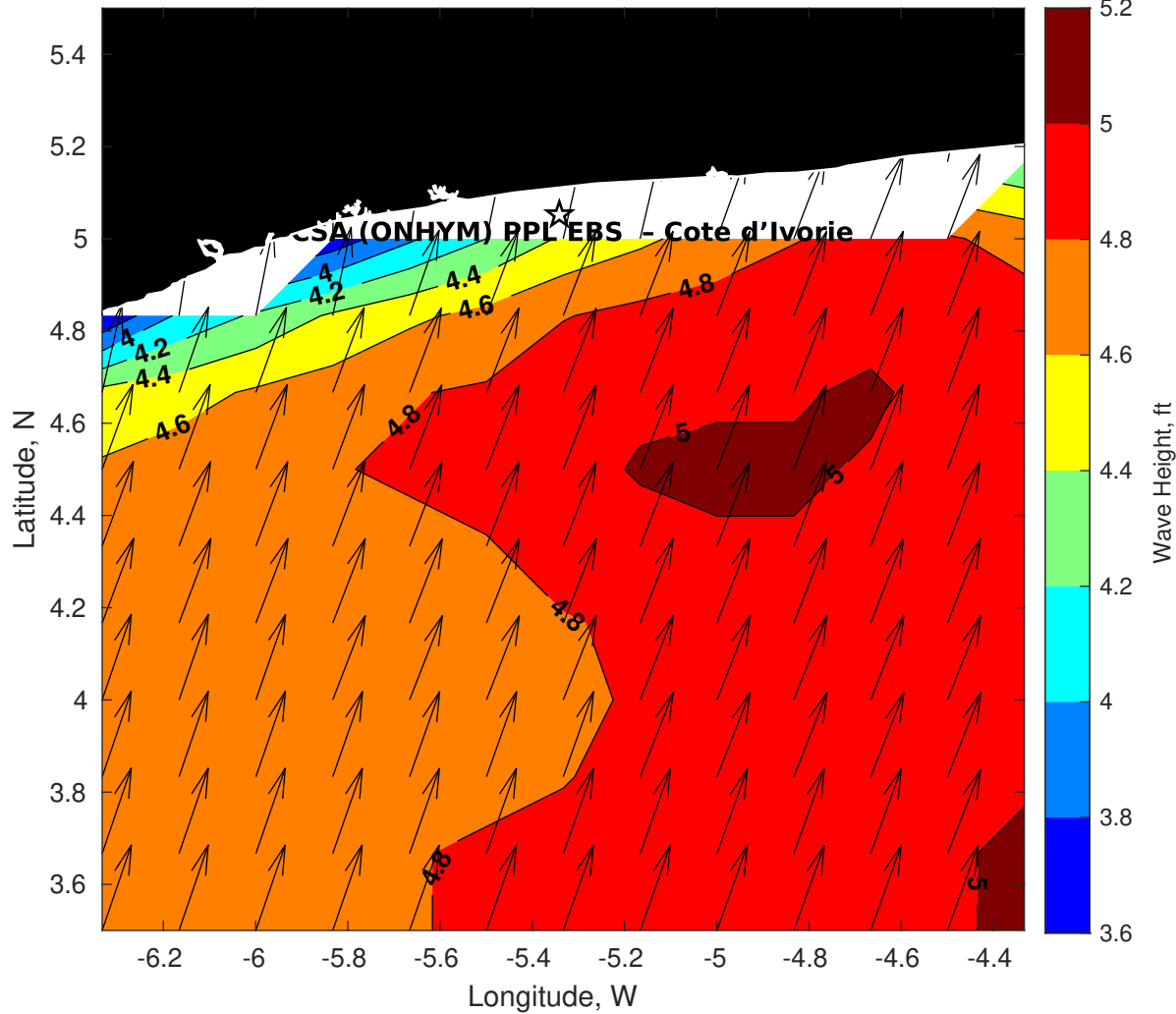
Wave Height (ft) for CSA (ONHYM) PPL EBS - Cote d'Ivoire at 17-Aug-2025 09:00:00
