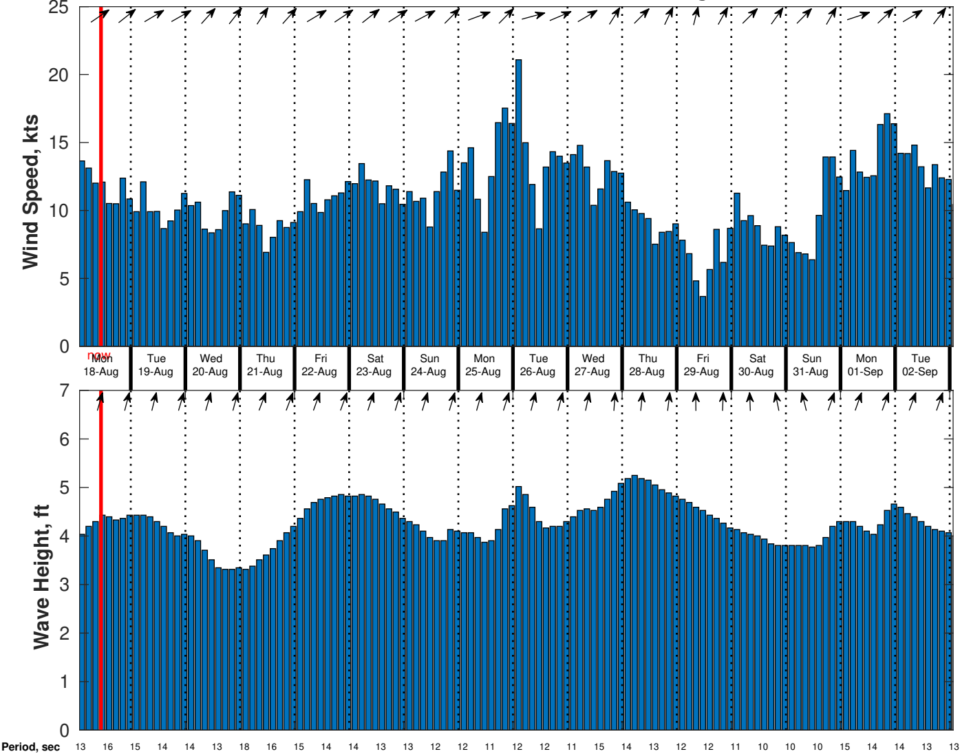
Wind & Wave Forecast for CSA (ONHYM) PPL EBS - Cote d'Ivoire from 17-Aug-2025 01:00:00 to 02-Sep-2025 01:00:00
