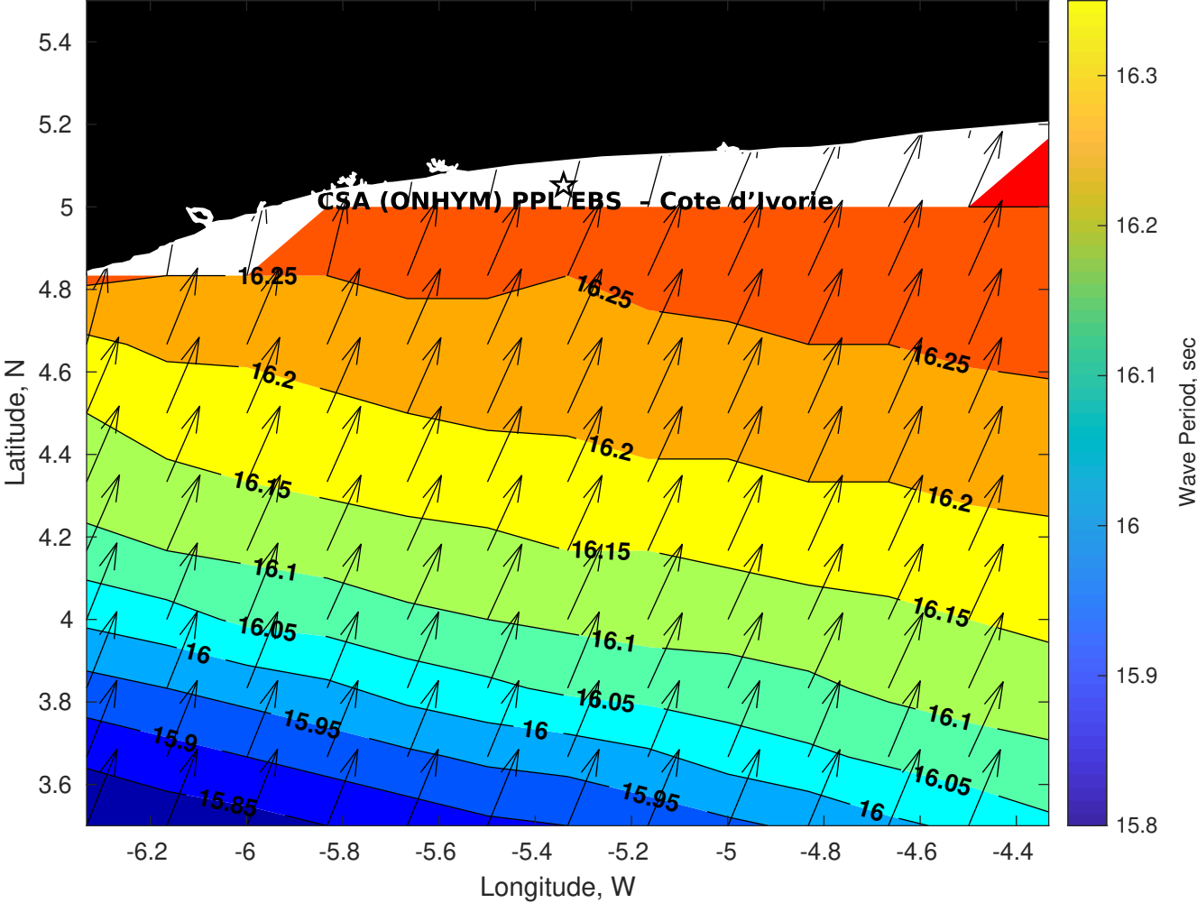
Wave Period (sec) for CSA (ONHYM) PPL EBS - Cote d'Ivoire at 17-Aug-2025 09:00:00
