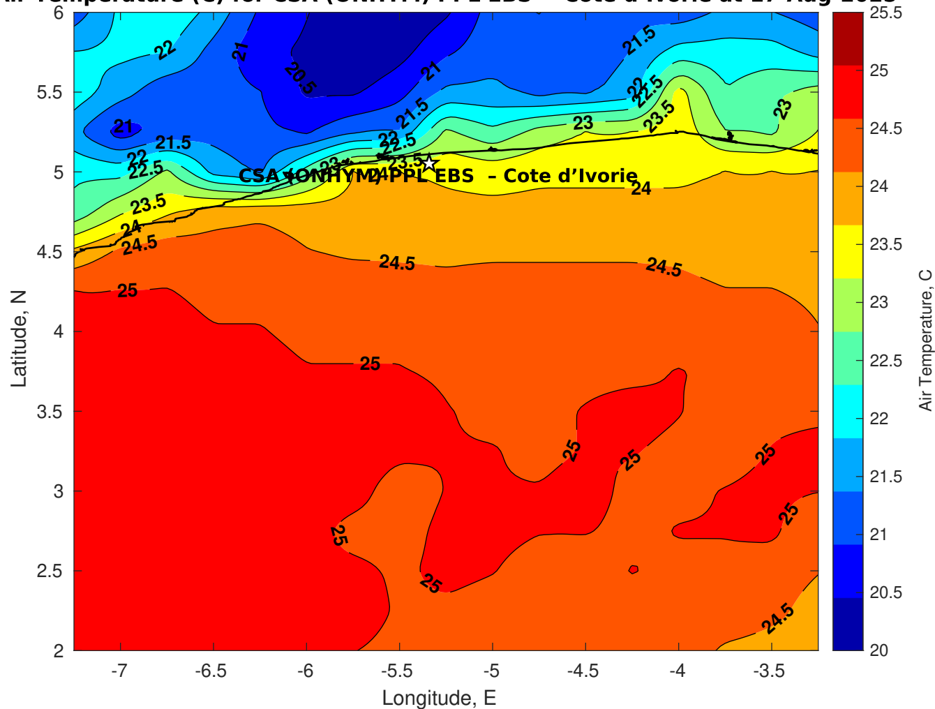
Air Temperature (C) for CSA (ONHYM) PPL EBS - Cote d'Ivoire at 17-Aug-2025
