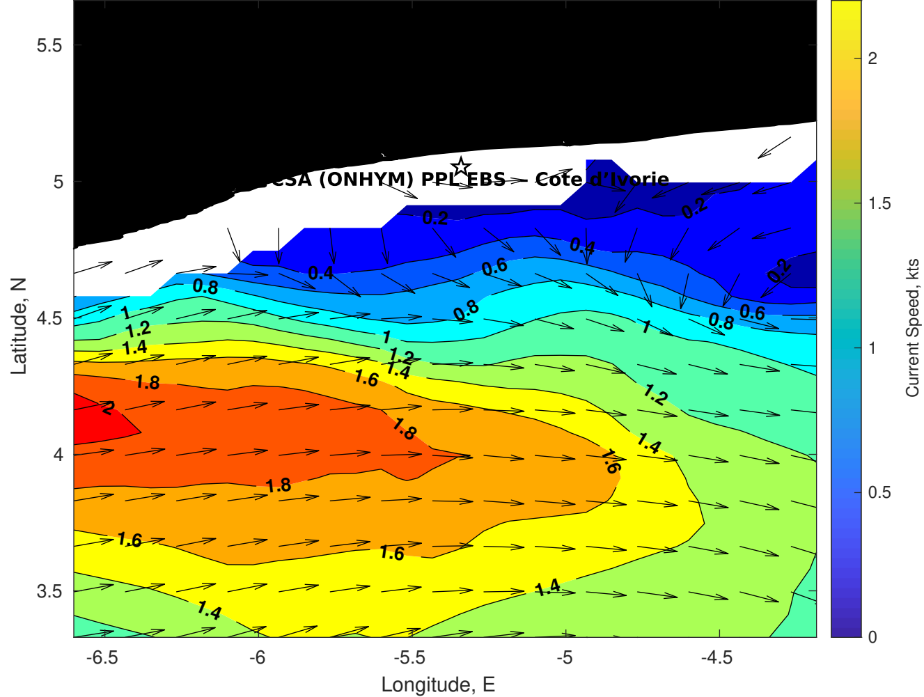
Surface Currents for CSA (ONHYM) PPL EBS - Cote d'Ivoire at 16-Aug-2025 00:00:00
