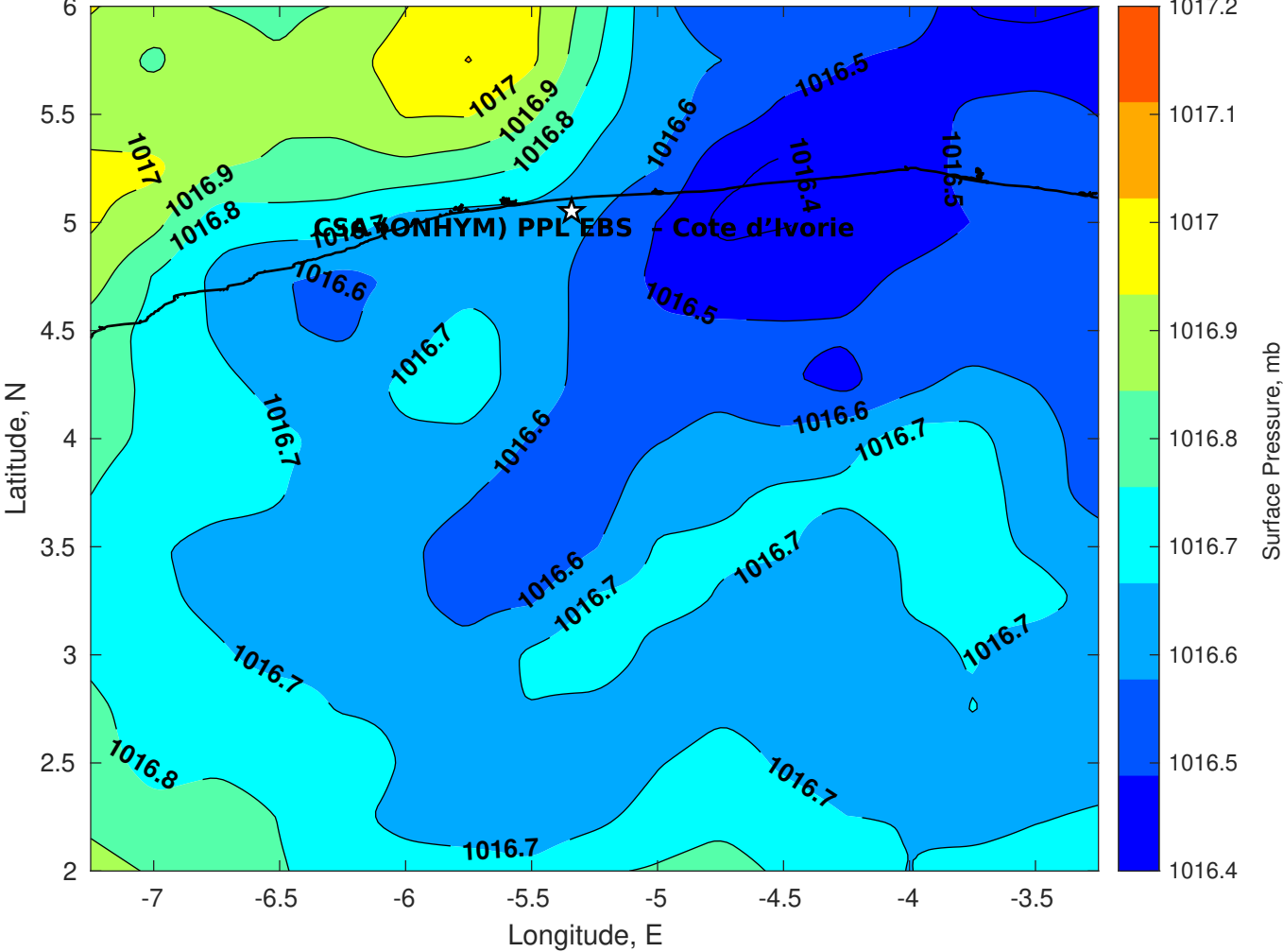
Surface Pressure (mb) for CSA (ONHYM) PPL EBS - Cote d'Ivoire at 19-Aug-2025 00:00:00
