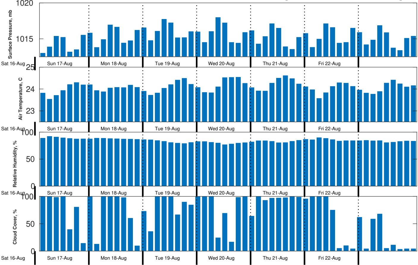
Met Forecast for CSA (ONHYM) PPL EBS - Cote d'Ivoire from 17-Aug-2025 00:00:00 to 24-Aug-2025 00:00:00
