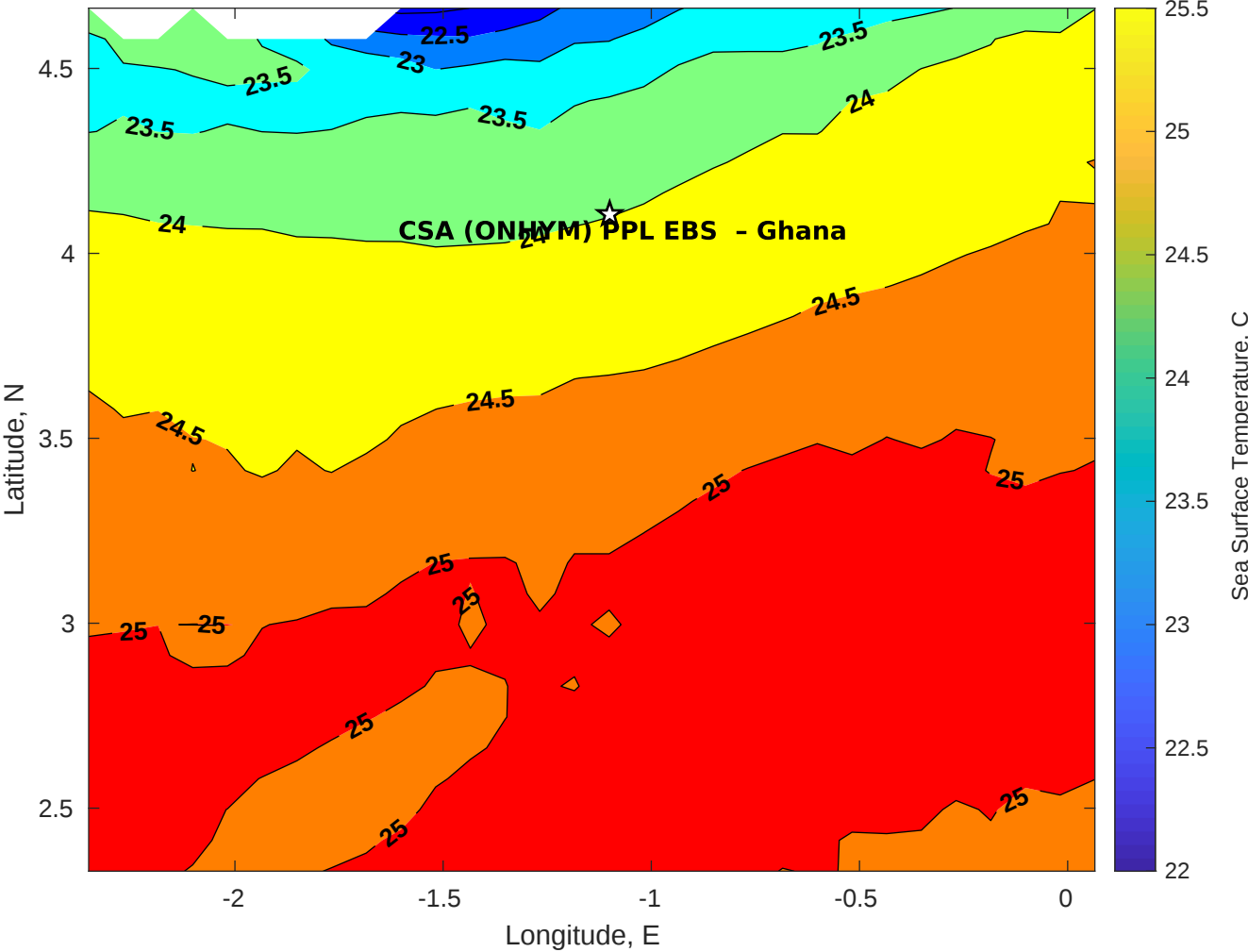
SST for CSA (ONHYM) PPL EBS - Ghana at 16-Aug-2025 00:00:00
