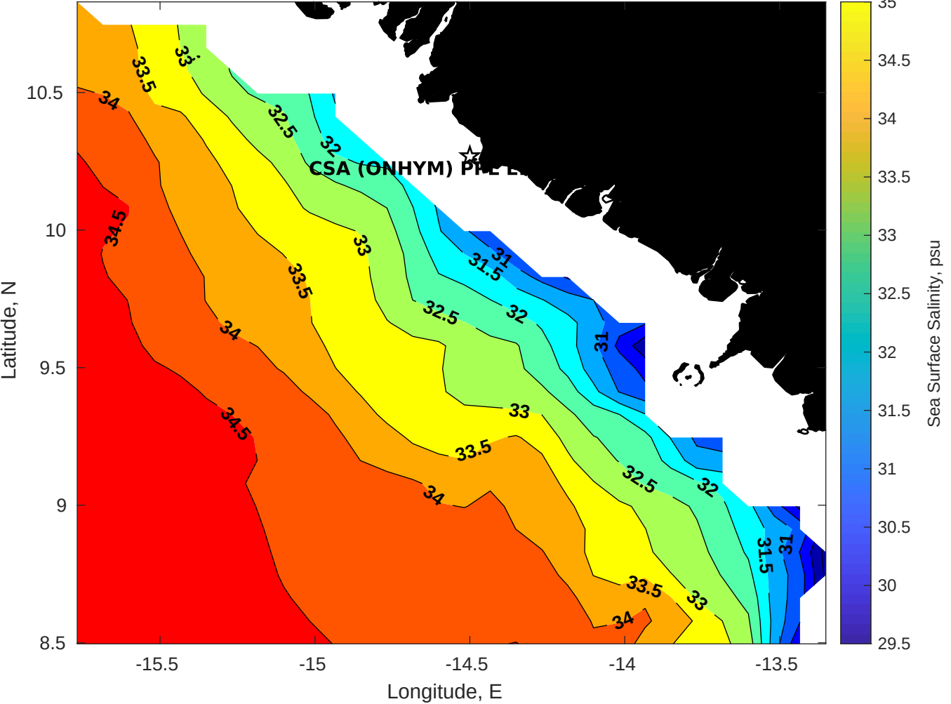
Surface Salinity for CSA (ONHYM) PPL EBS - Guinea at 16-Aug-2025 00:00:00
