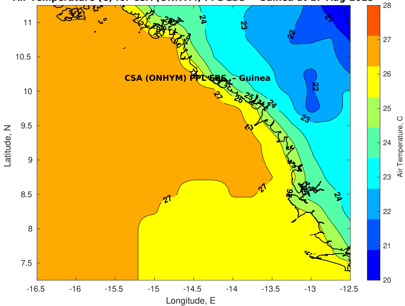
Air Temperature (C) for CSA (ONHYM) PPL EBS - Guinea at 17-Aug-2025
