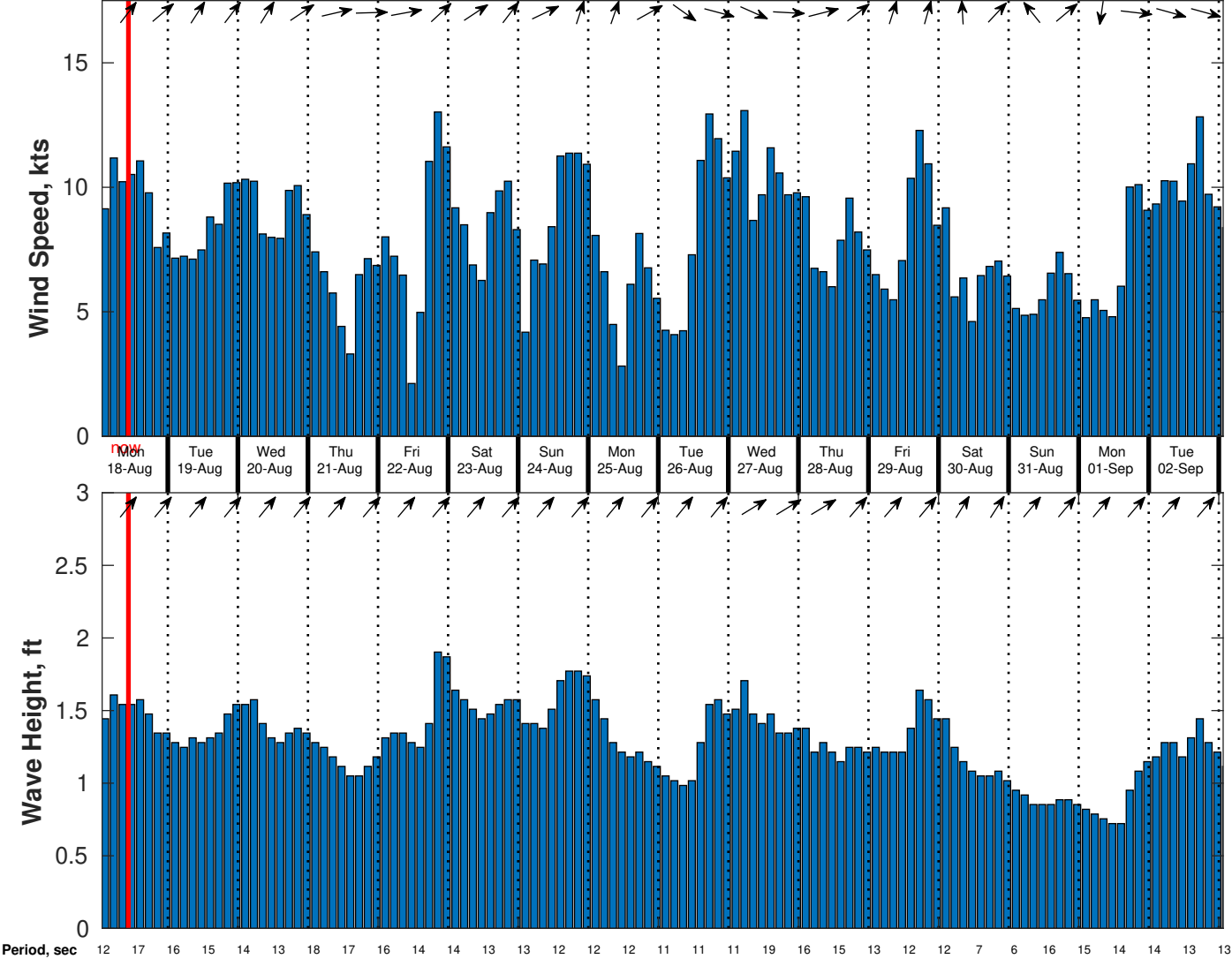
Wind & Wave Forecast for CSA (ONHYM) PPL EBS - Guinea from 17-Aug-2025 01:00:00 to 02-Sep-2025 01:00:00
