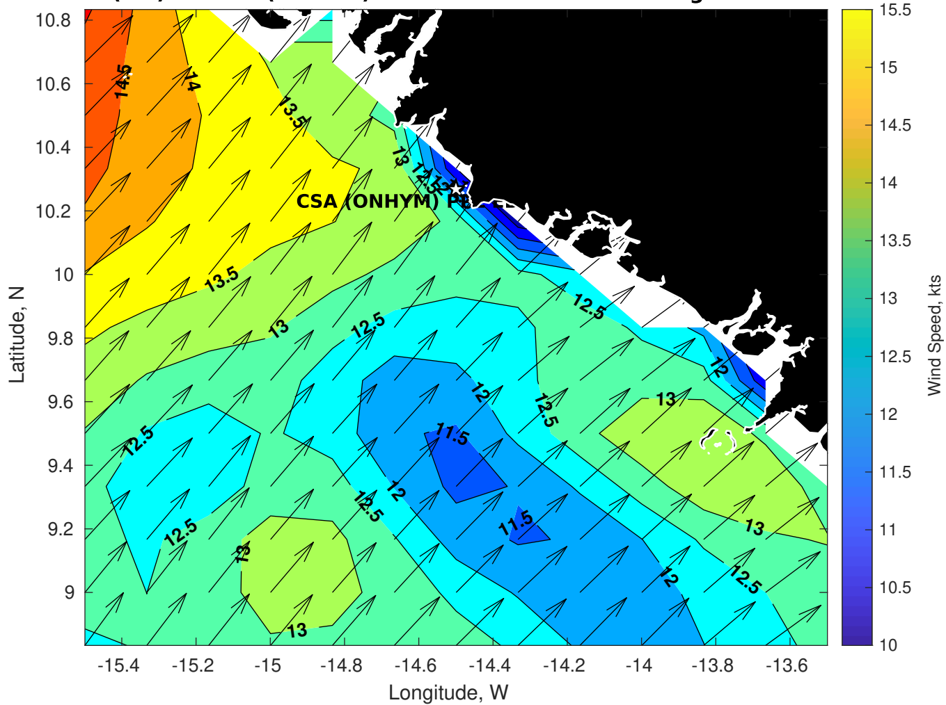
Winds (kts) for CSA (ONHYM) PPL EBS - Guinea at 17-Aug-2025 09:00:00
