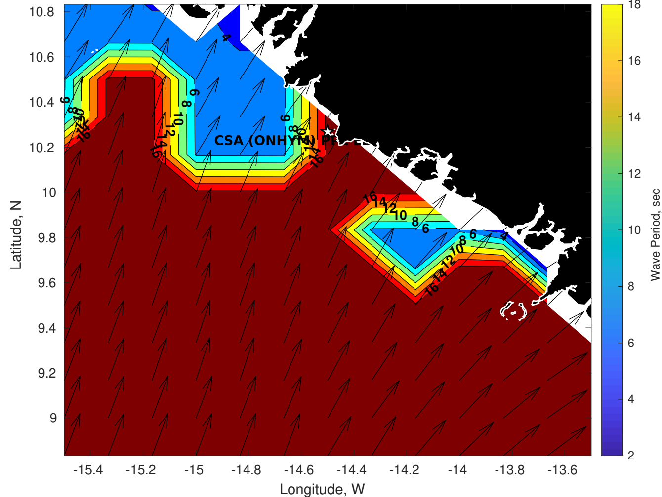
Wave Period (sec) for CSA (ONHYM) PPL EBS - Guinea at 17-Aug-2025 09:00:00
