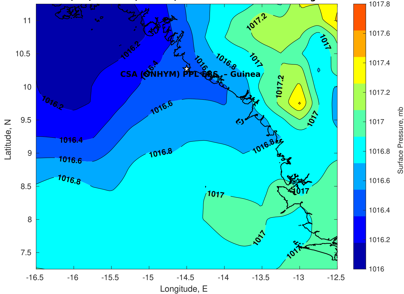
Surface Pressure (mb) for CSA (ONHYM) PPL EBS - Guinea at 19-Aug-2025 00:00:00
