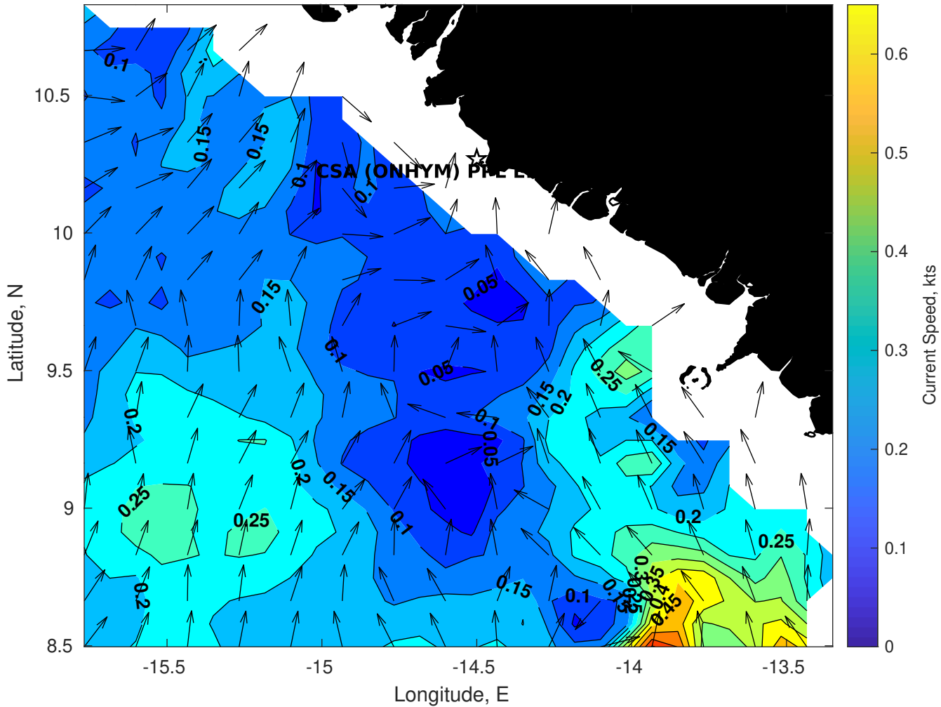
Surface Currents for CSA (ONHYM) PPL EBS - Guinea at 16-Aug-2025 00:00:00
