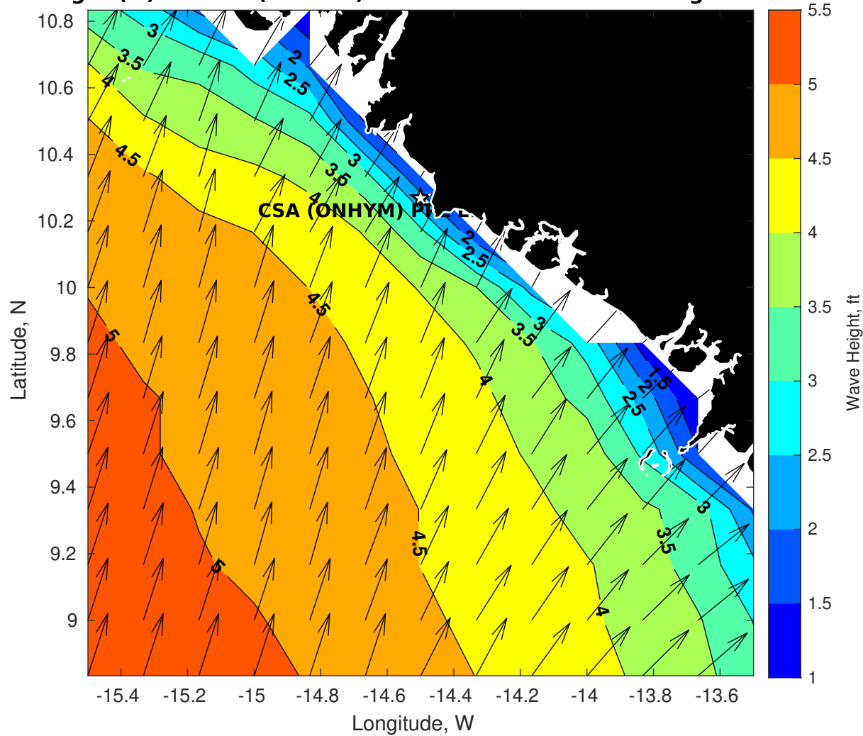
Wave Height (ft) for CSA (ONHYM) PPL EBS - Guinea at 17-Aug-2025 09:00:00
