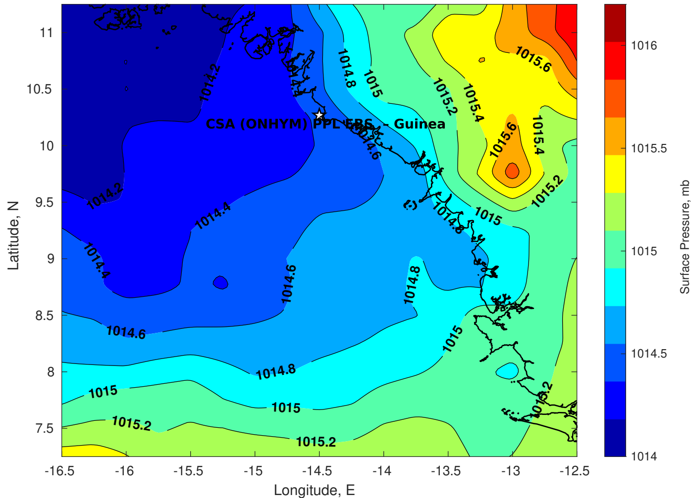
Surface Pressure (mb) for CSA (ONHYM) PPL EBS - Guinea at 18-Aug-2025 00:00:00
