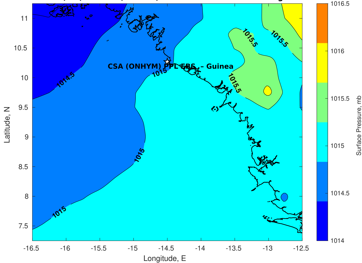
Surface Pressure (mb) for CSA (ONHYM) PPL EBS - Guinea at 17-Aug-2025 00:00:00
