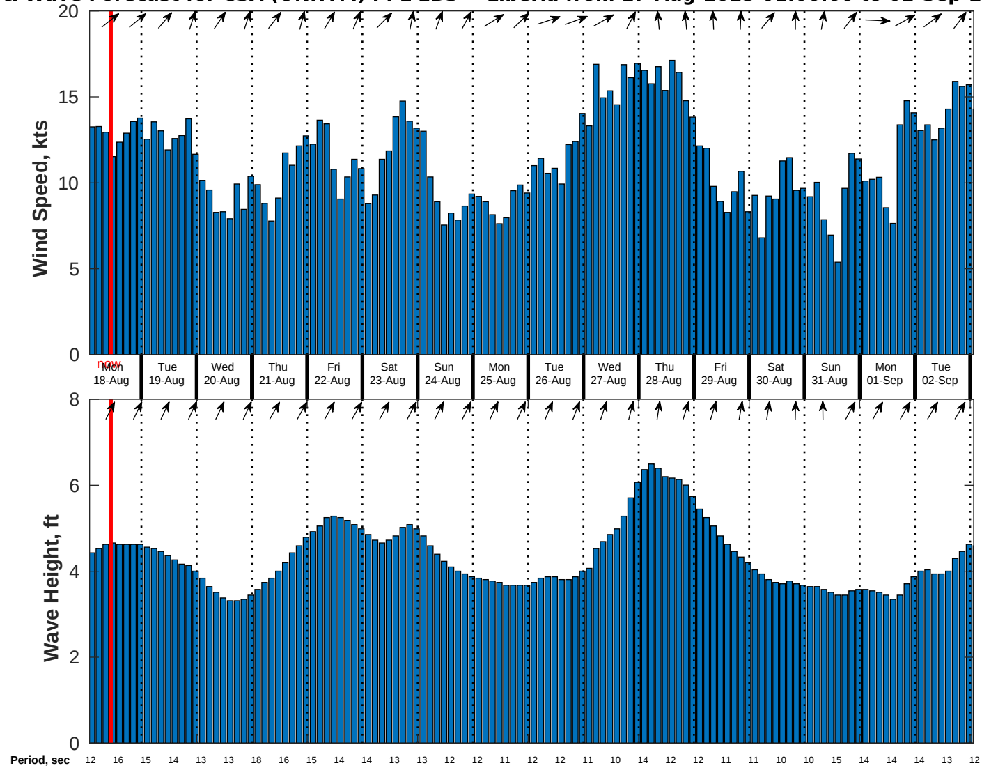
Wind & Wave Forecast for CSA (ONHYM) PPL EBS - Liberia from 17-Aug-2025 01:00:00 to 02-Sep-2025 01:00:00
