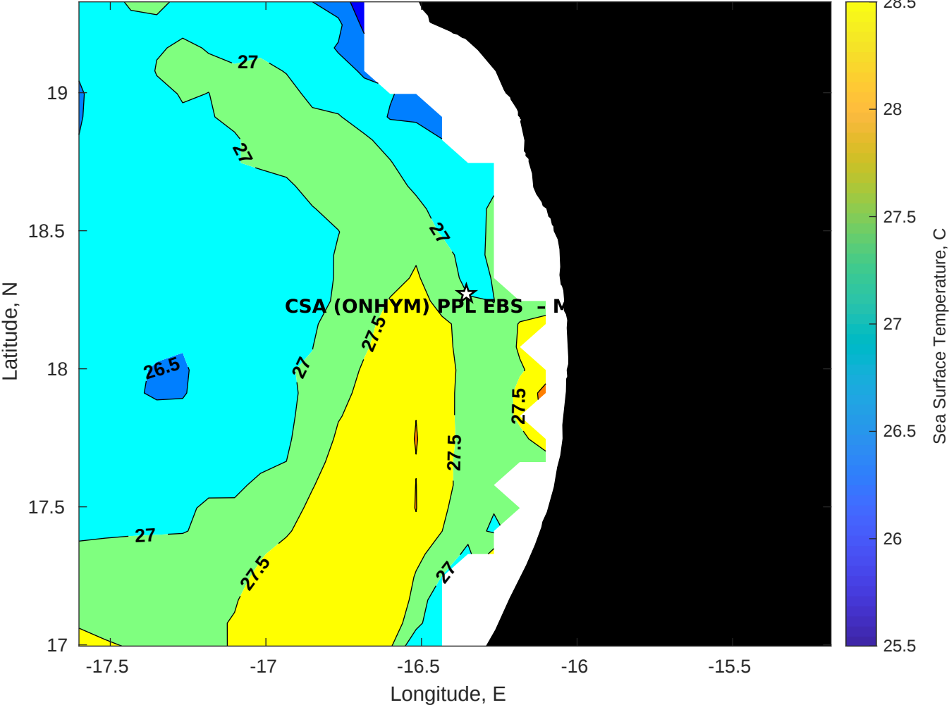
SST for CSA (ONHYM) PPL EBS - Mauritania at 16-Aug-2025 00:00:00
