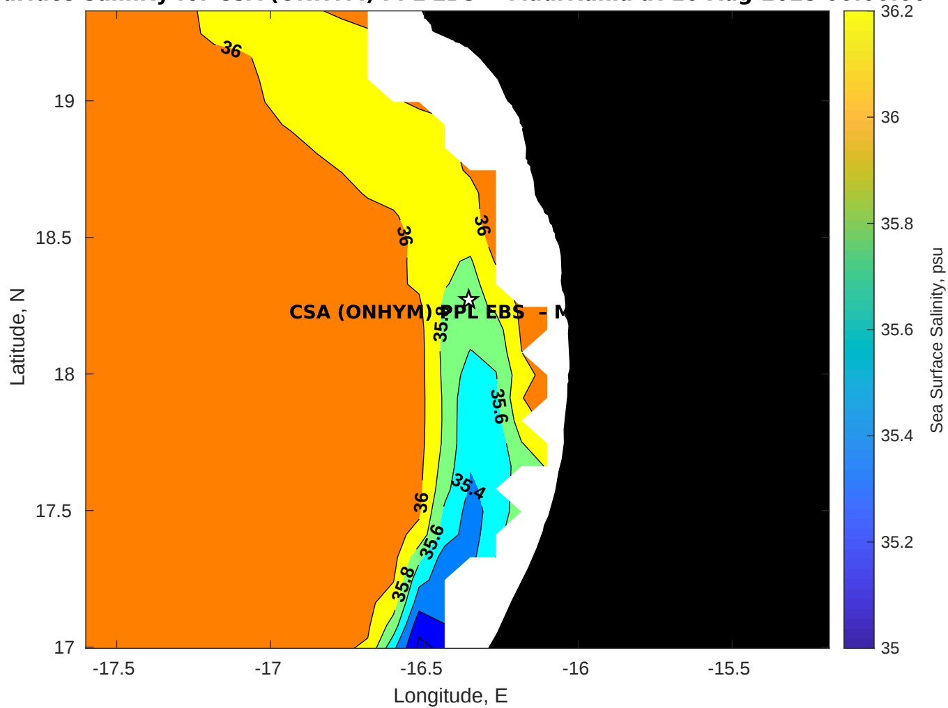
Surface Salinity for CSA (ONHYM) PPL EBS - Mauritania at 16-Aug-2025 00:00:00
