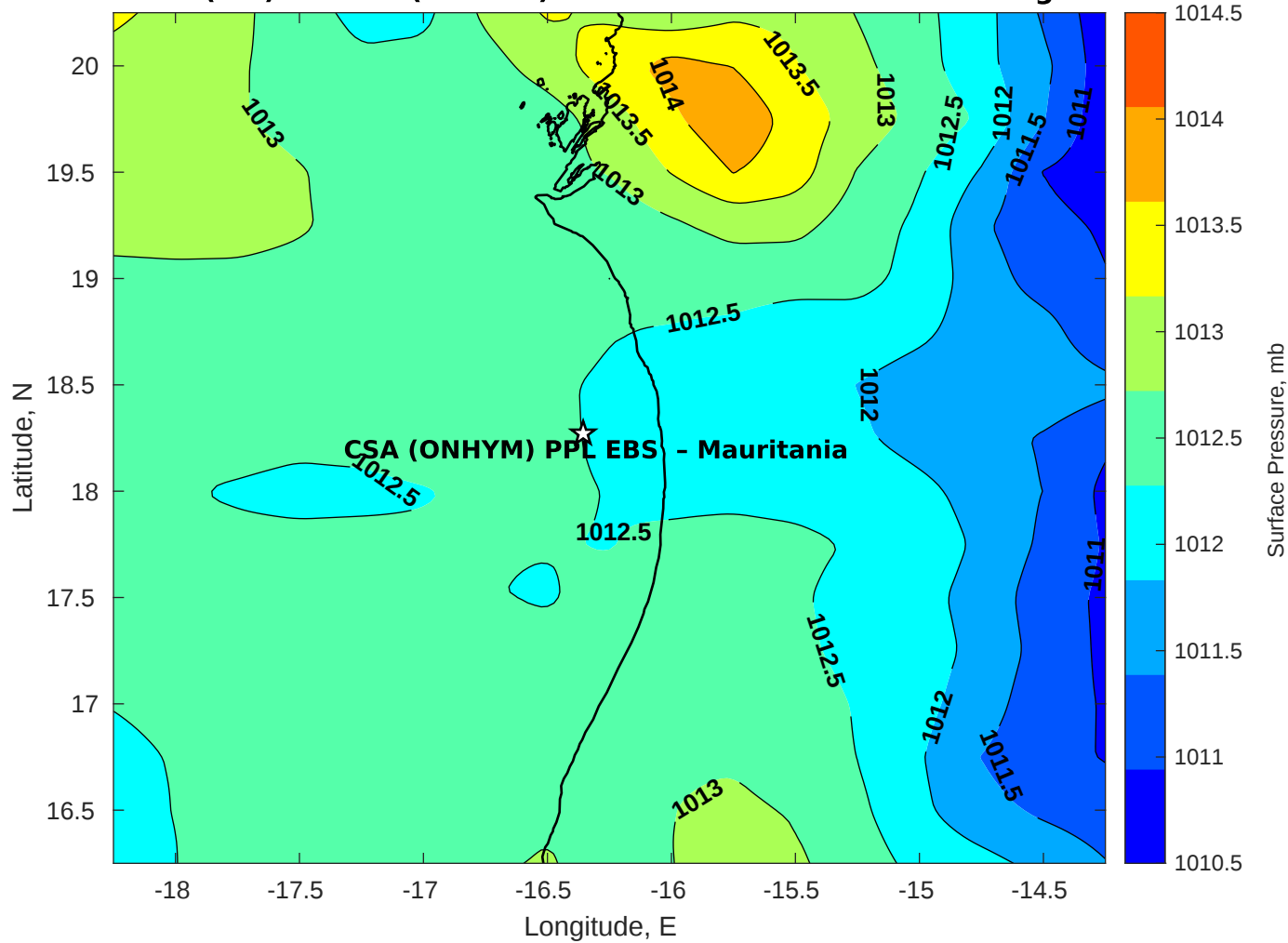
Surface Pressure (mb) for CSA (ONHYM) PPL EBS - Mauritania at 18-Aug-2025 00:00:00
