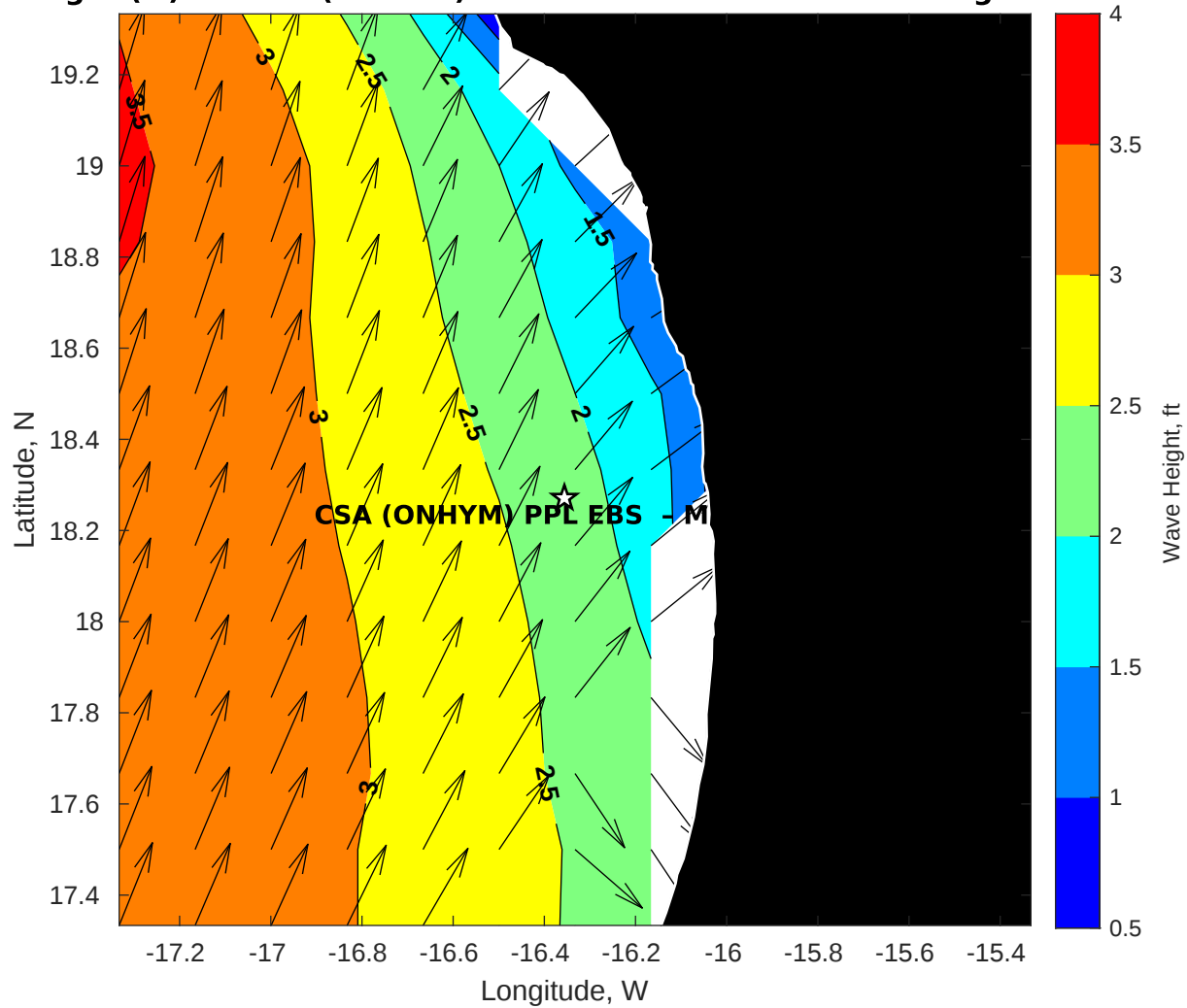
Wave Height (ft) for CSA (ONHYM) PPL EBS - Mauritania at 17-Aug-2025 09:00:00
