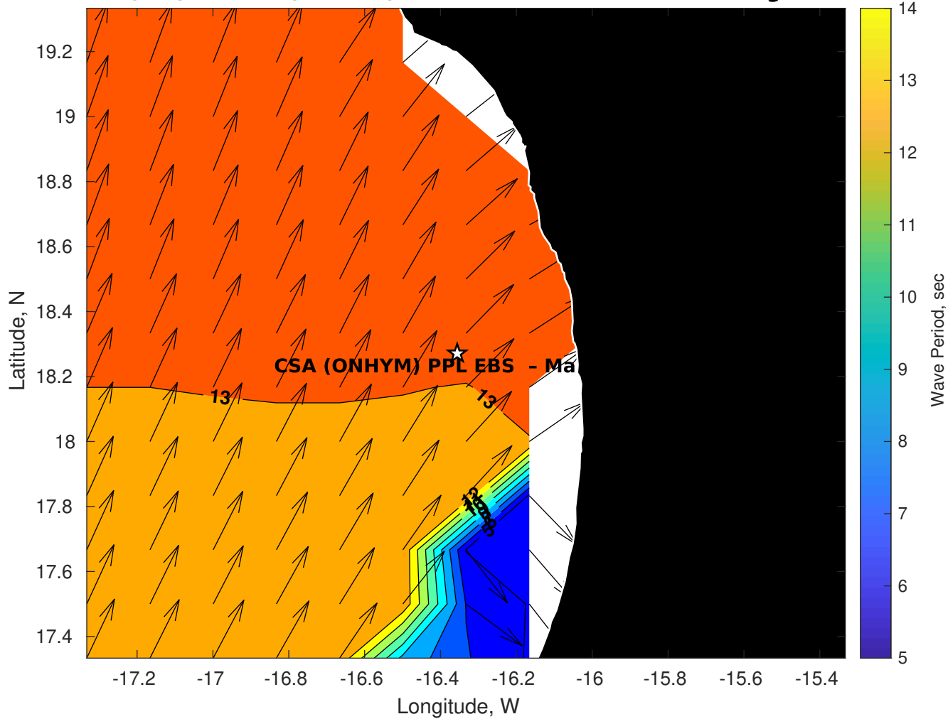
Wave Period (sec) for CSA (ONHYM) PPL EBS - Mauritania at 17-Aug-2025 09:00:00
