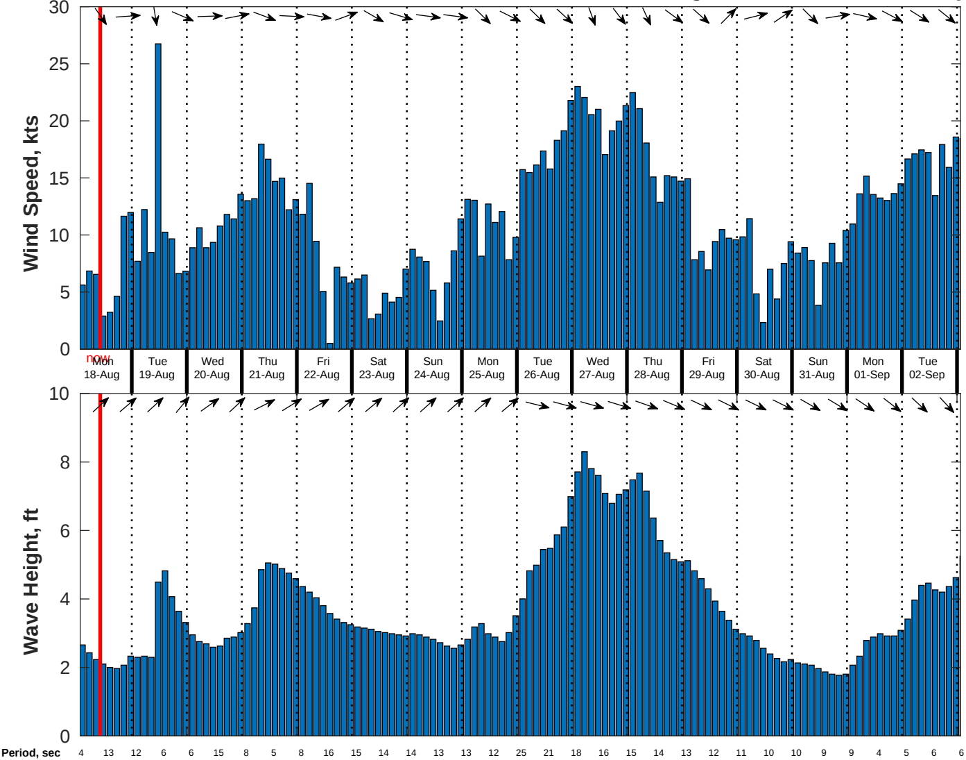
Wind & Wave Forecast for CSA (ONHYM) PPL EBS - Mauritania from 17-Aug-2025 01:00:00 to 02-Sep-2025 01:00:00
