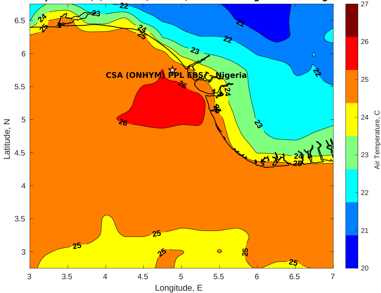
Air Temperature (C) for CSA (ONHYM) PPL EBS - Nigeria at 17-Aug-2025
