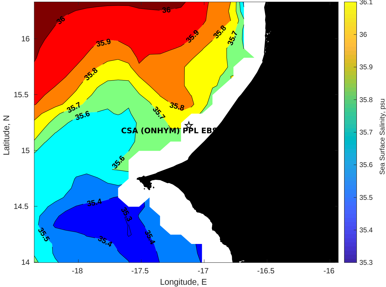
Surface Salinity for CSA (ONHYM) PPL EBS - Senegal at 16-Aug-2025 00:00:00
