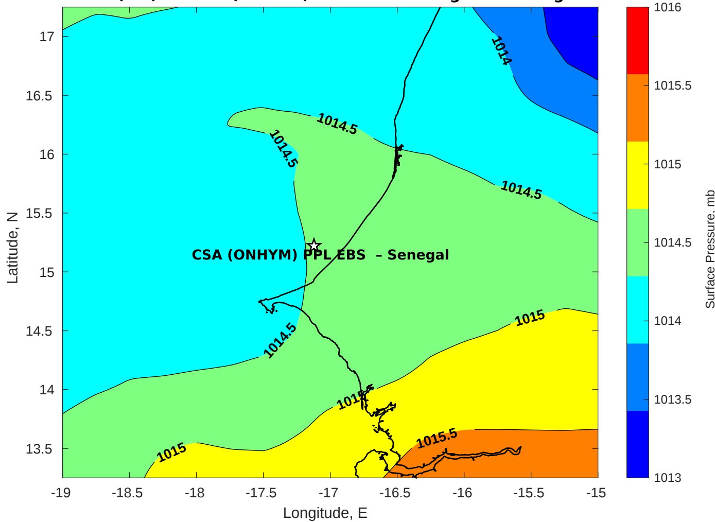
Surface Pressure (mb) for CSA (ONHYM) PPL EBS - Senegal at 19-Aug-2025 00:00:00
