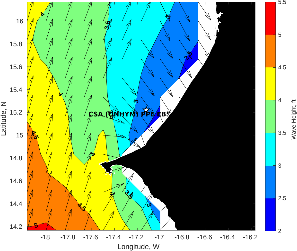
Wave Height (ft) for CSA (ONHYM) PPL EBS - Senegal at 17-Aug-2025 09:00:00
