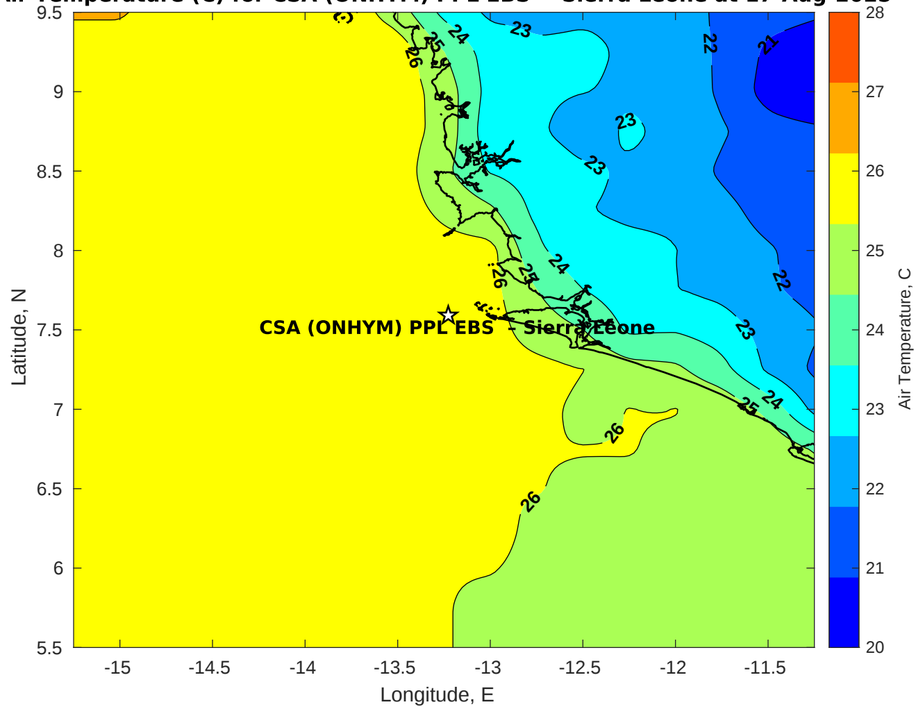
Air Temperature (C) for CSA (ONHYM) PPL EBS - Sierra Leone at 17-Aug-2025
