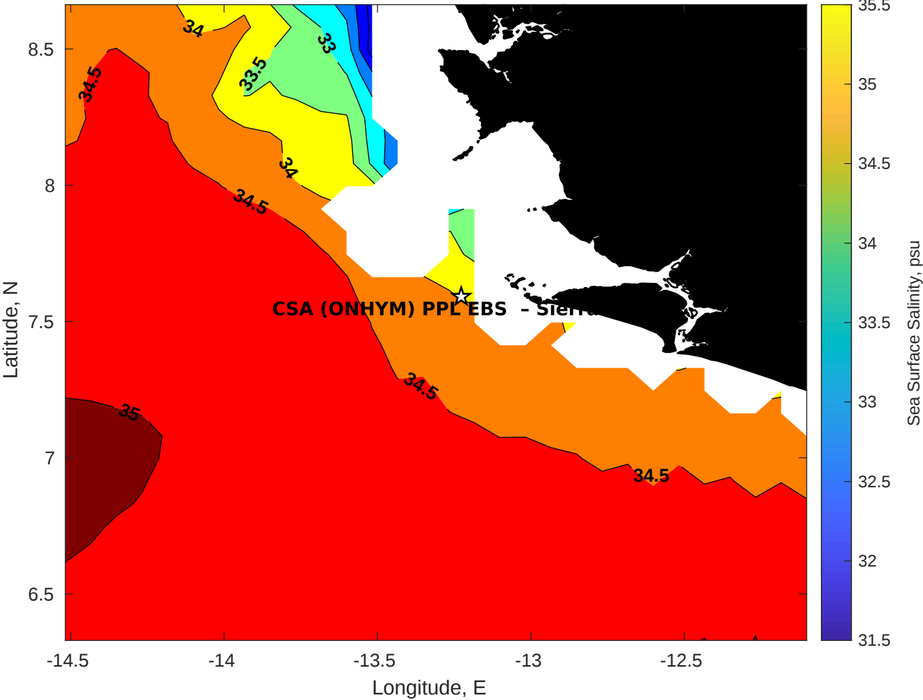
Surface Salinity for CSA (ONHYM) PPL EBS - Sierra Leone at 16-Aug-2025 00:00:00
