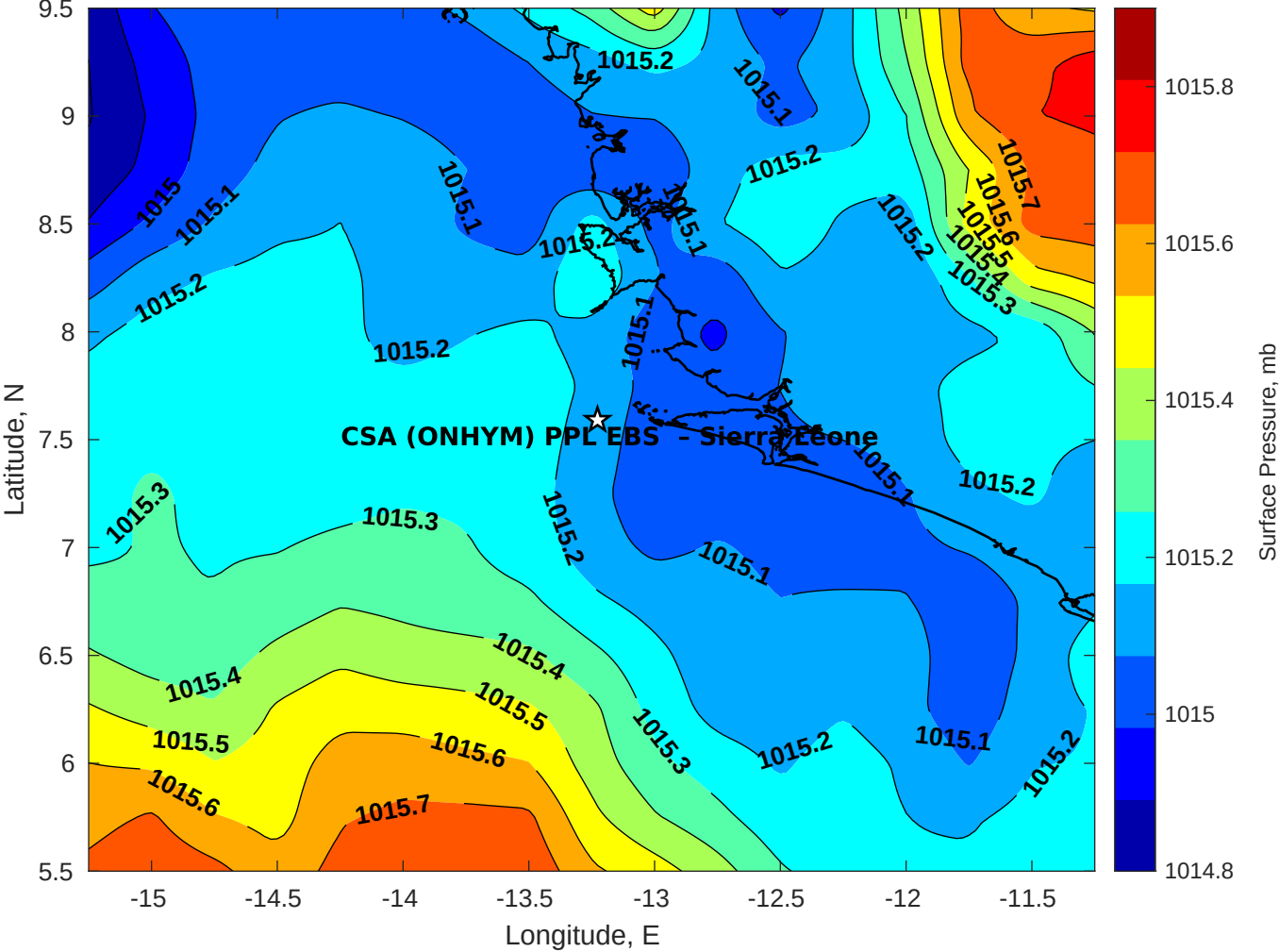
Surface Pressure (mb) for CSA (ONHYM) PPL EBS - Sierra Leone at 17-Aug-2025 00:00:00
