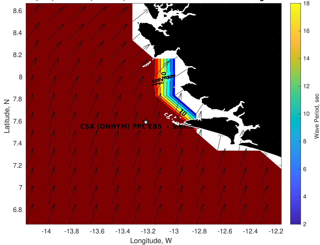
Wave Period (sec) for CSA (ONHYM) PPL EBS - Sierra Leone at 17-Aug-2025 09:00:00
