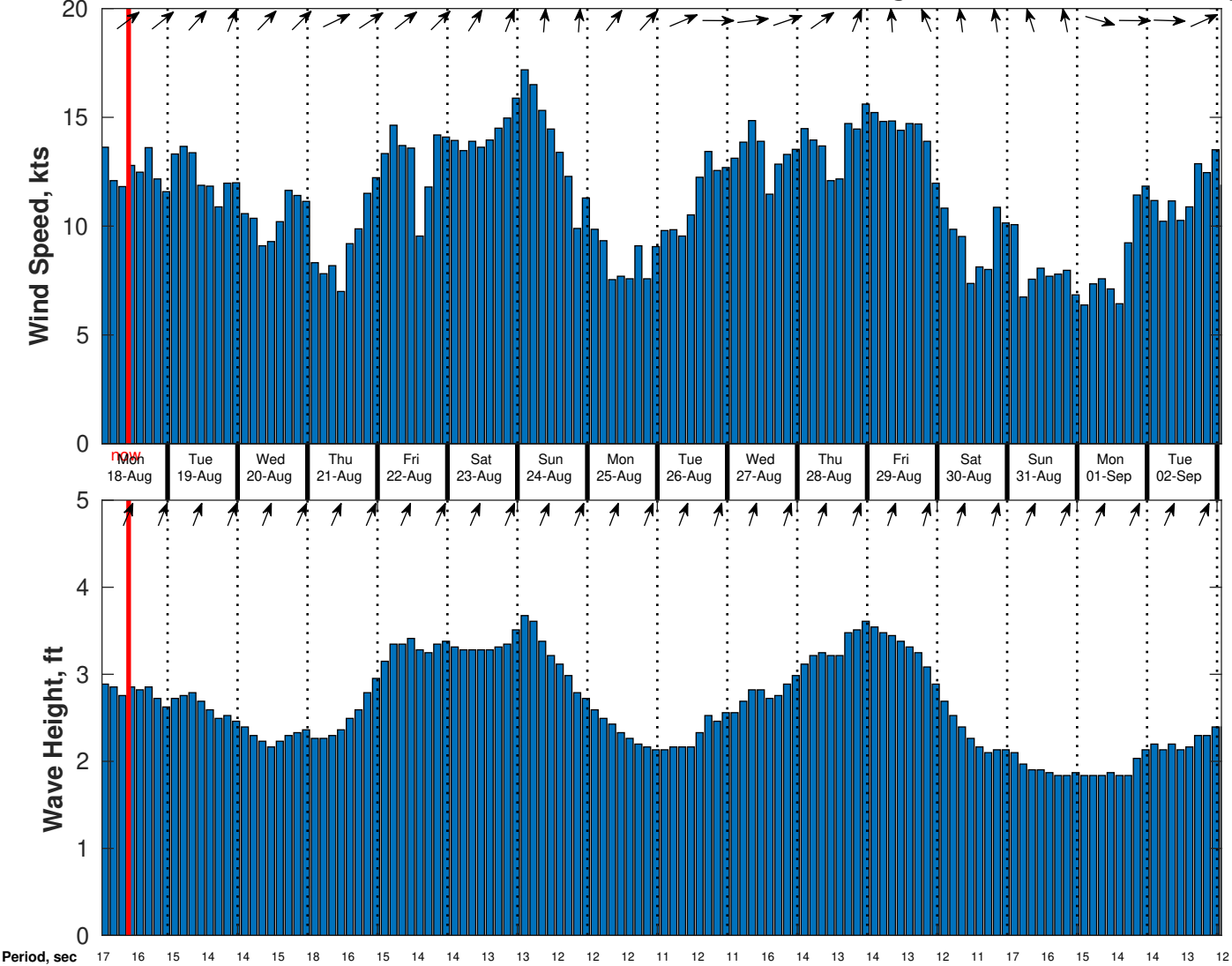
Wind & Wave Forecast for CSA (ONHYM) PPL EBS - Sierra Leone from 17-Aug-2025 01:00:00 to 02-Sep-2025 01:00:00
