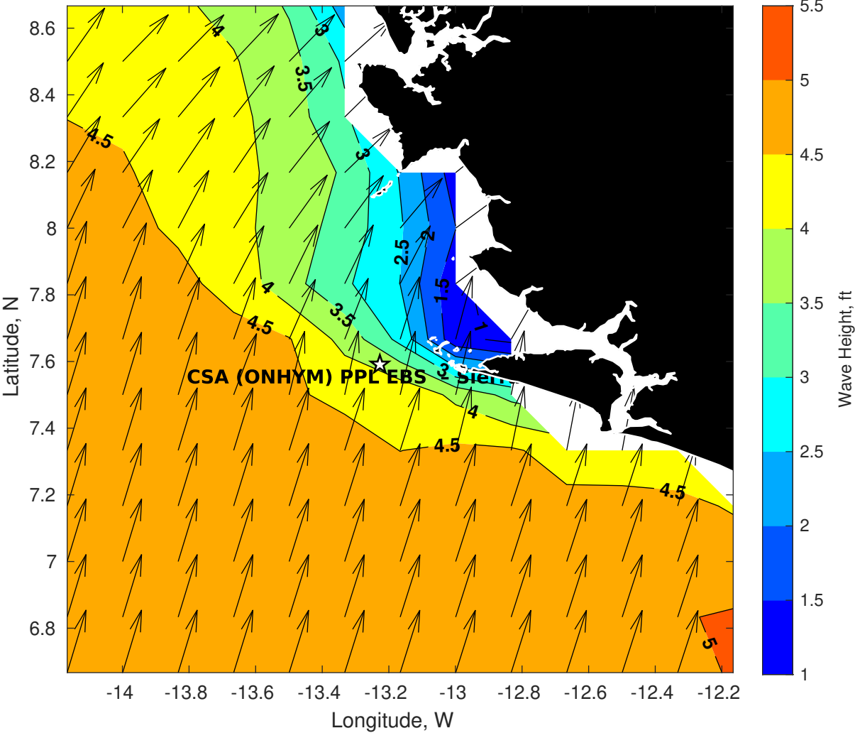
Wave Height (ft) for CSA (ONHYM) PPL EBS - Sierra Leone at 17-Aug-2025 09:00:00
