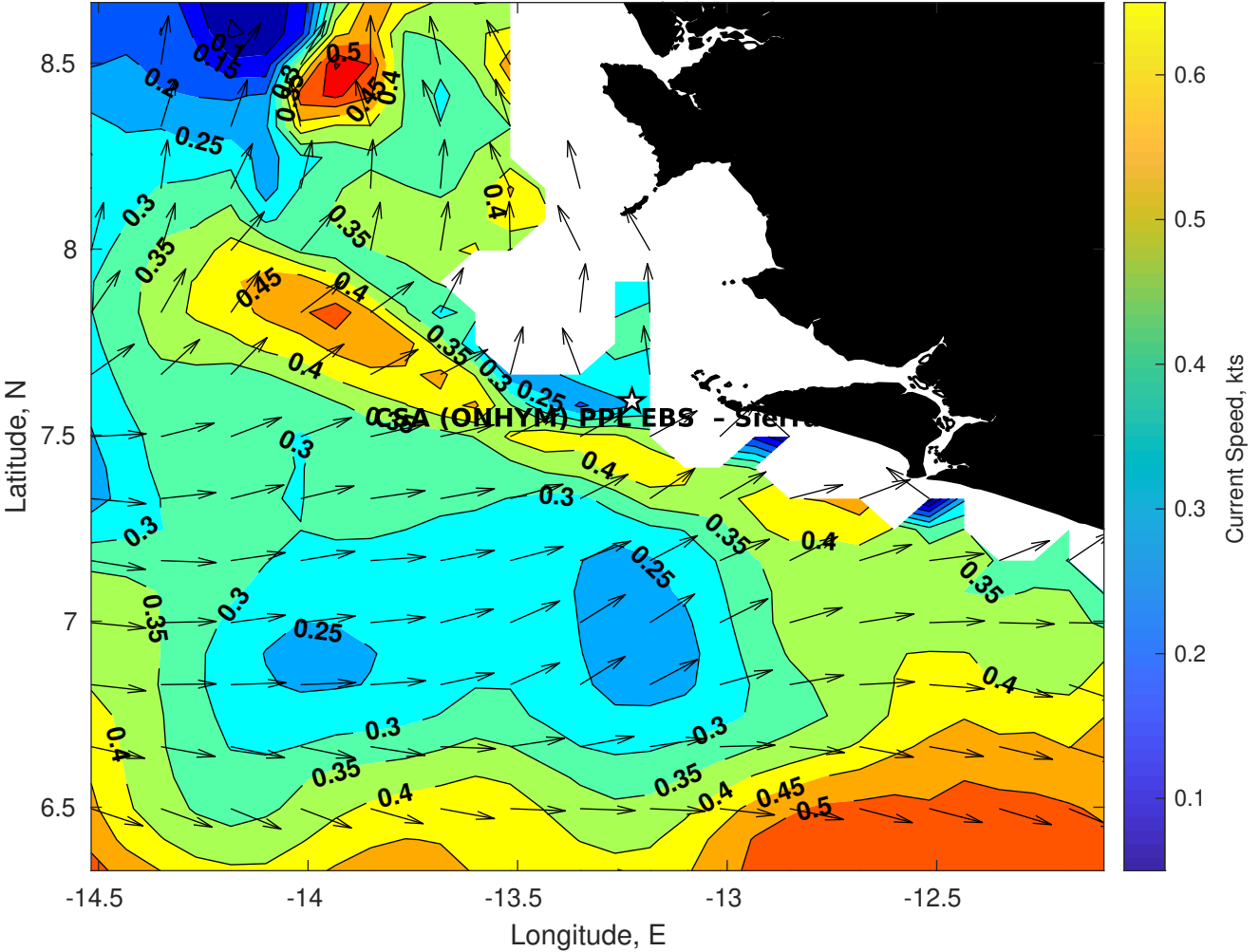
Surface Currents for CSA (ONHYM) PPL EBS - Sierra Leone at 16-Aug-2025 00:00:00
