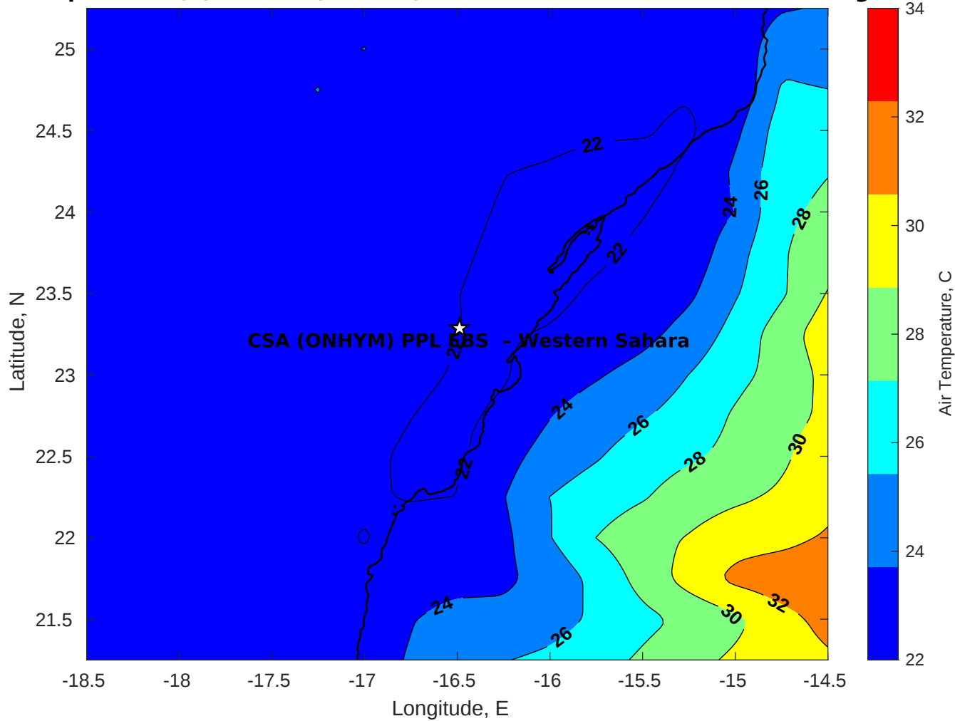
Air Temperature (C) for CSA (ONHYM) PPL EBS - Western Sahara at 17-Aug-2025
