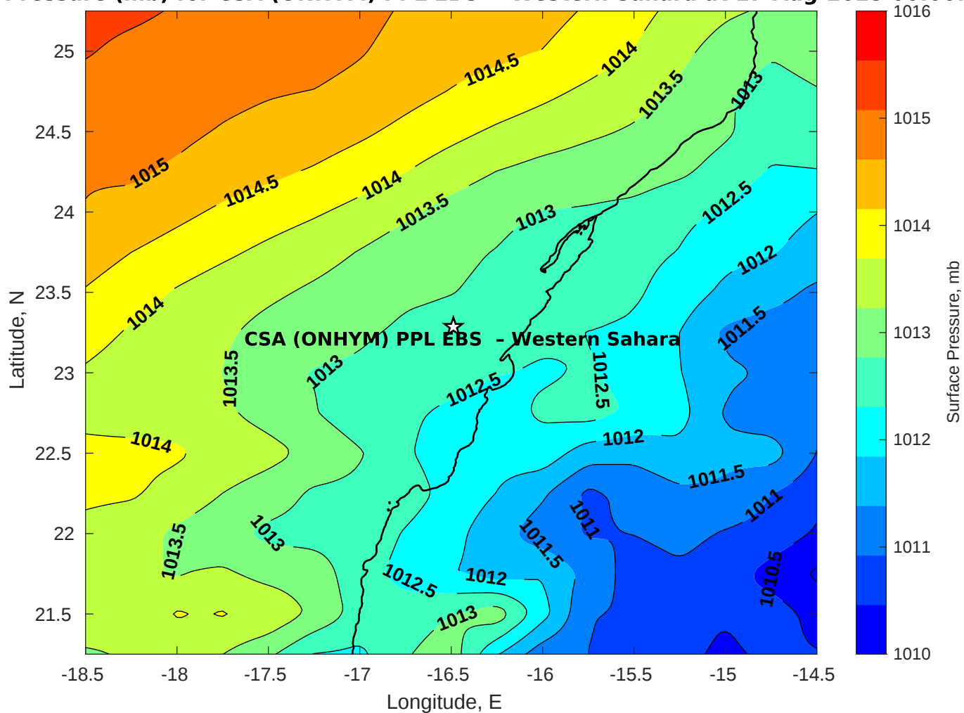
Surface Pressure (mb) for CSA (ONHYM) PPL EBS - Western Sahara at 17-Aug-2025 00:00:00
