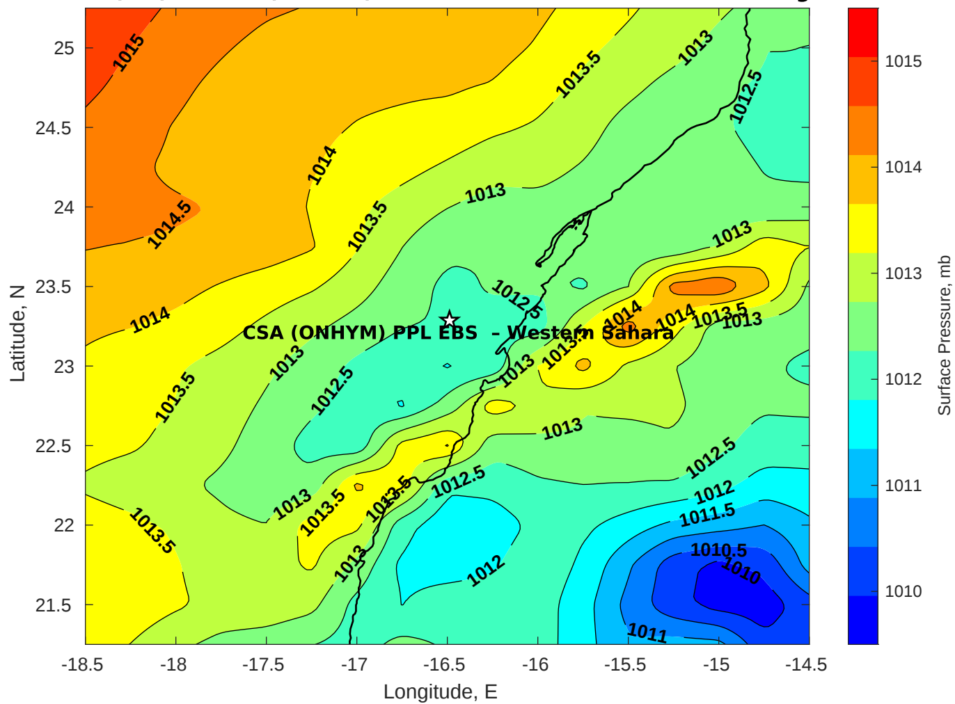
Surface Pressure (mb) for CSA (ONHYM) PPL EBS - Western Sahara at 18-Aug-2025 00:00:00
