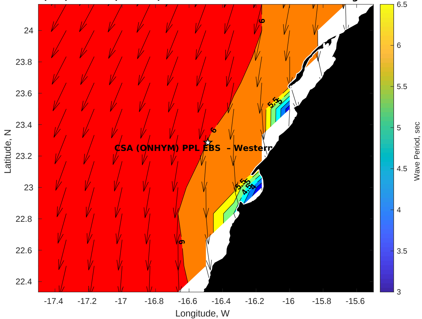
Wave Period (sec) for CSA (ONHYM) PPL EBS - Western Sahara at 17-Aug-2025 09:00:00
