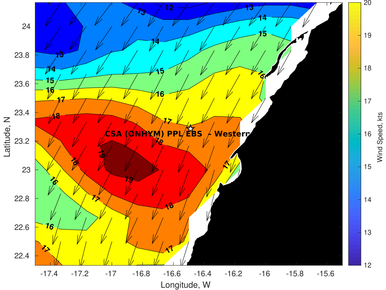
Winds (kts) for CSA (ONHYM) PPL EBS - Western Sahara at 17-Aug-2025 09:00:00
