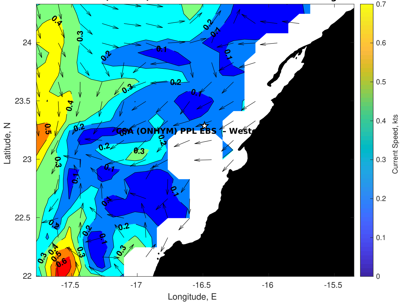
Surface Currents for CSA (ONHYM) PPL EBS - Western Sahara at 16-Aug-2025 00:00:00
