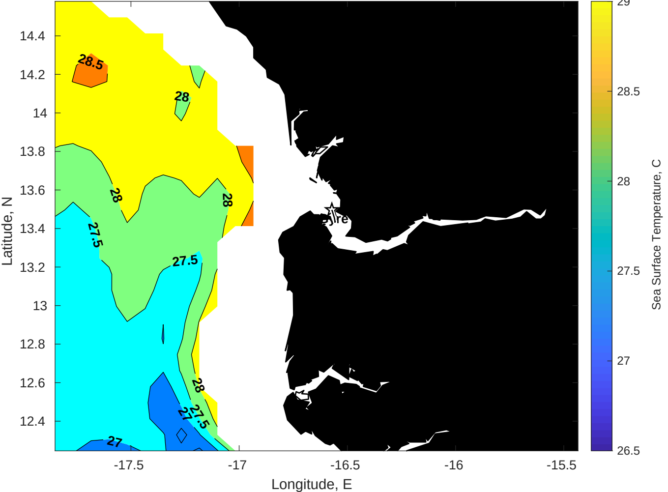
SST for Gyre at 16-Aug-2025 00:00:00
