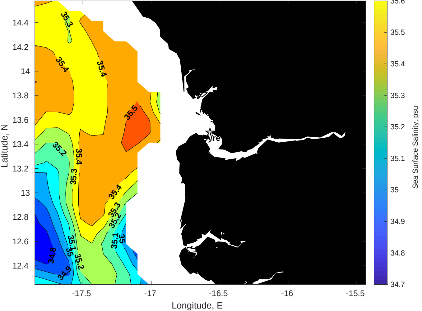
Surface Salinity for Gyre at 16-Aug-2025 00:00:00
