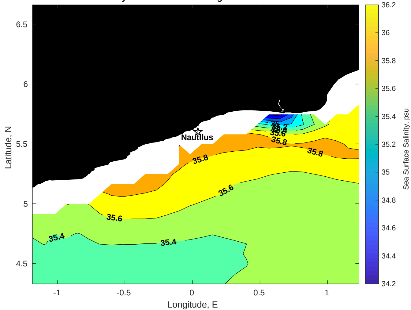
Surface Salinity for Nautilus at 16-Aug-2025 00:00:00
