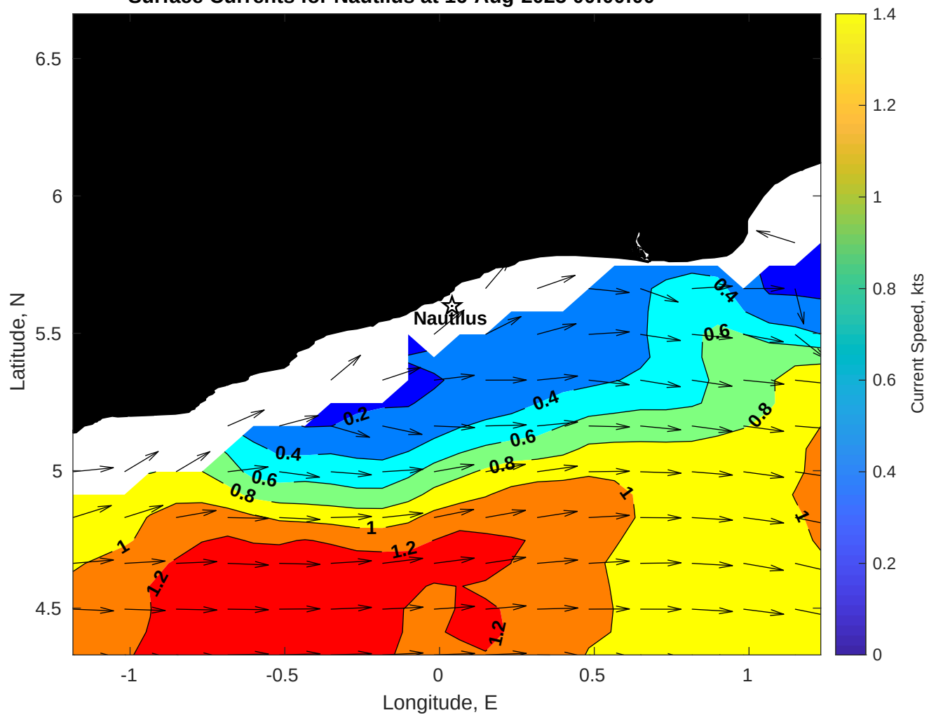
Surface Currents for Nautilus at 16-Aug-2025 00:00:00
