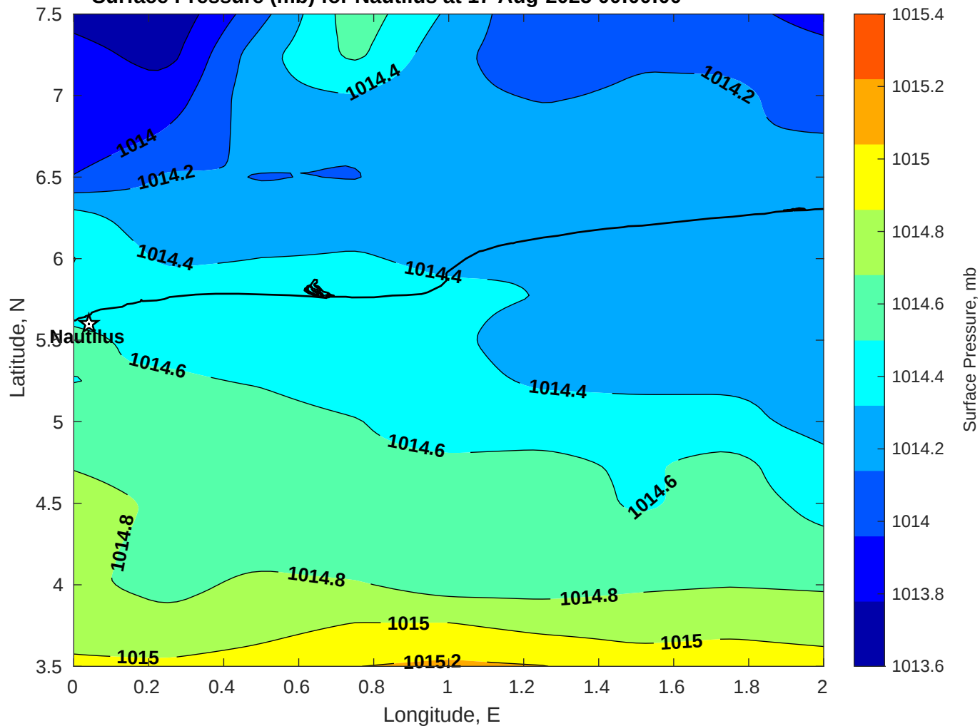
Surface Pressure (mb) for Nautilus at 17-Aug-2025 00:00:00
