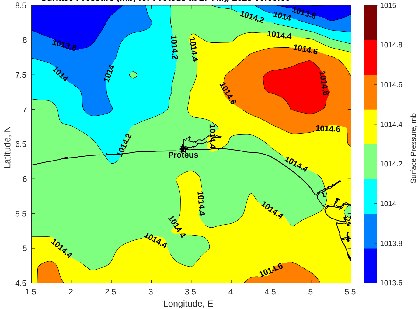
Surface Pressure (mb) for Proteus at 17-Aug-2025 00:00:00
