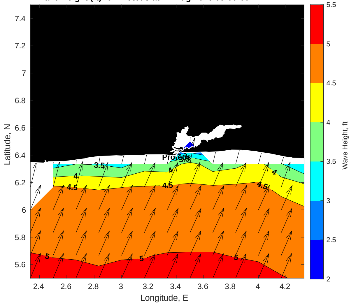
Wave Height (ft) for Proteus at 17-Aug-2025 09:00:00
