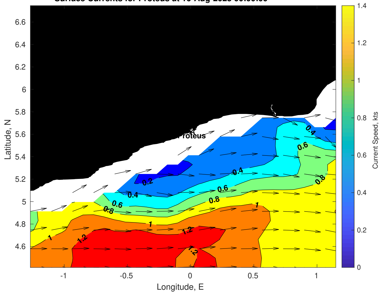
Surface Currents for Proteus at 16-Aug-2025 00:00:00
