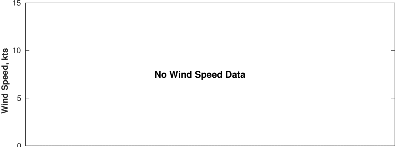
Wind & Wave Forecast for Proteus from 17-Aug-2025 01:00:00 to 02-Sep-2025 01:00:00
