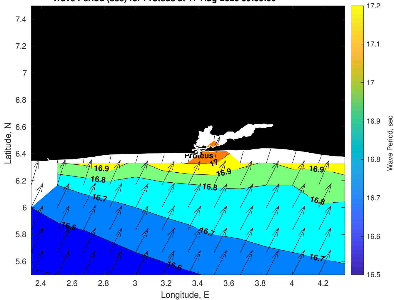
Wave Period (sec) for Proteus at 17-Aug-2025 09:00:00
