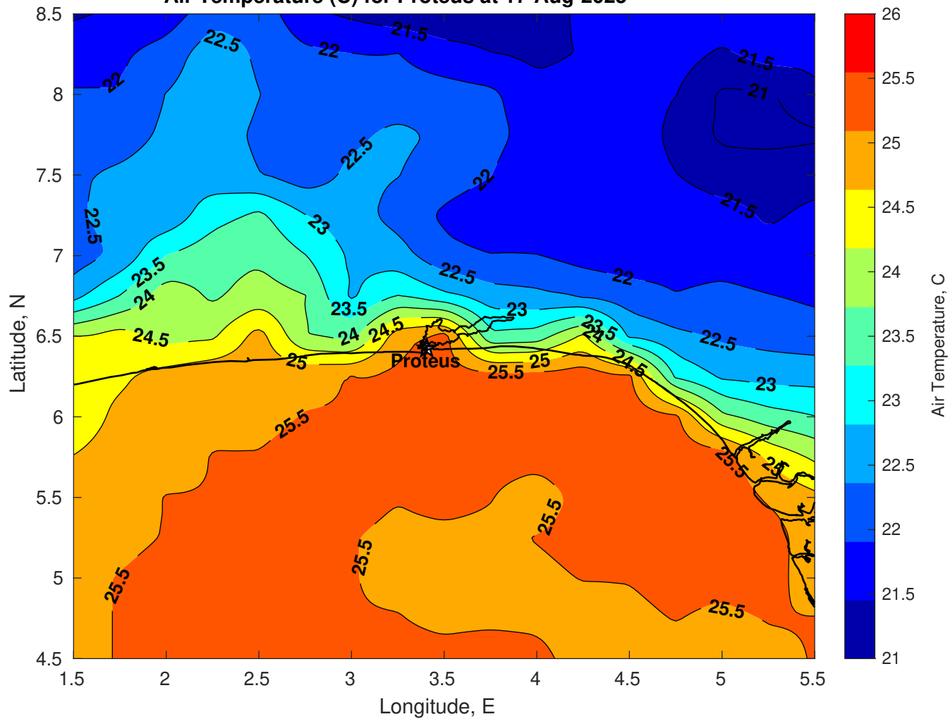
Air Temperature (C) for Proteus at 17-Aug-2025
