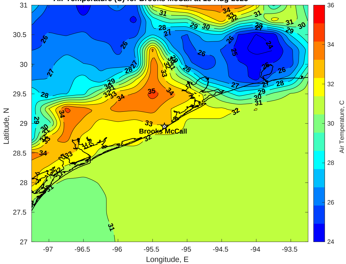
Air Temperature (C) for Brooks McCall at 18-Aug-2025
