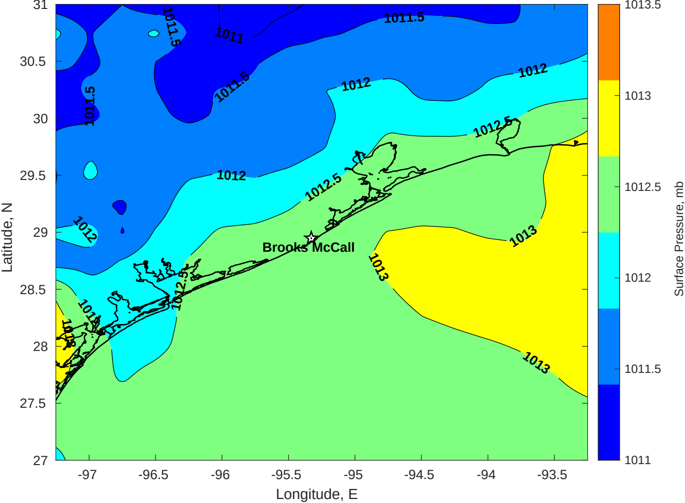
Surface Pressure (mb) for Brooks McCall at 20-Aug-2025 00:00:00
