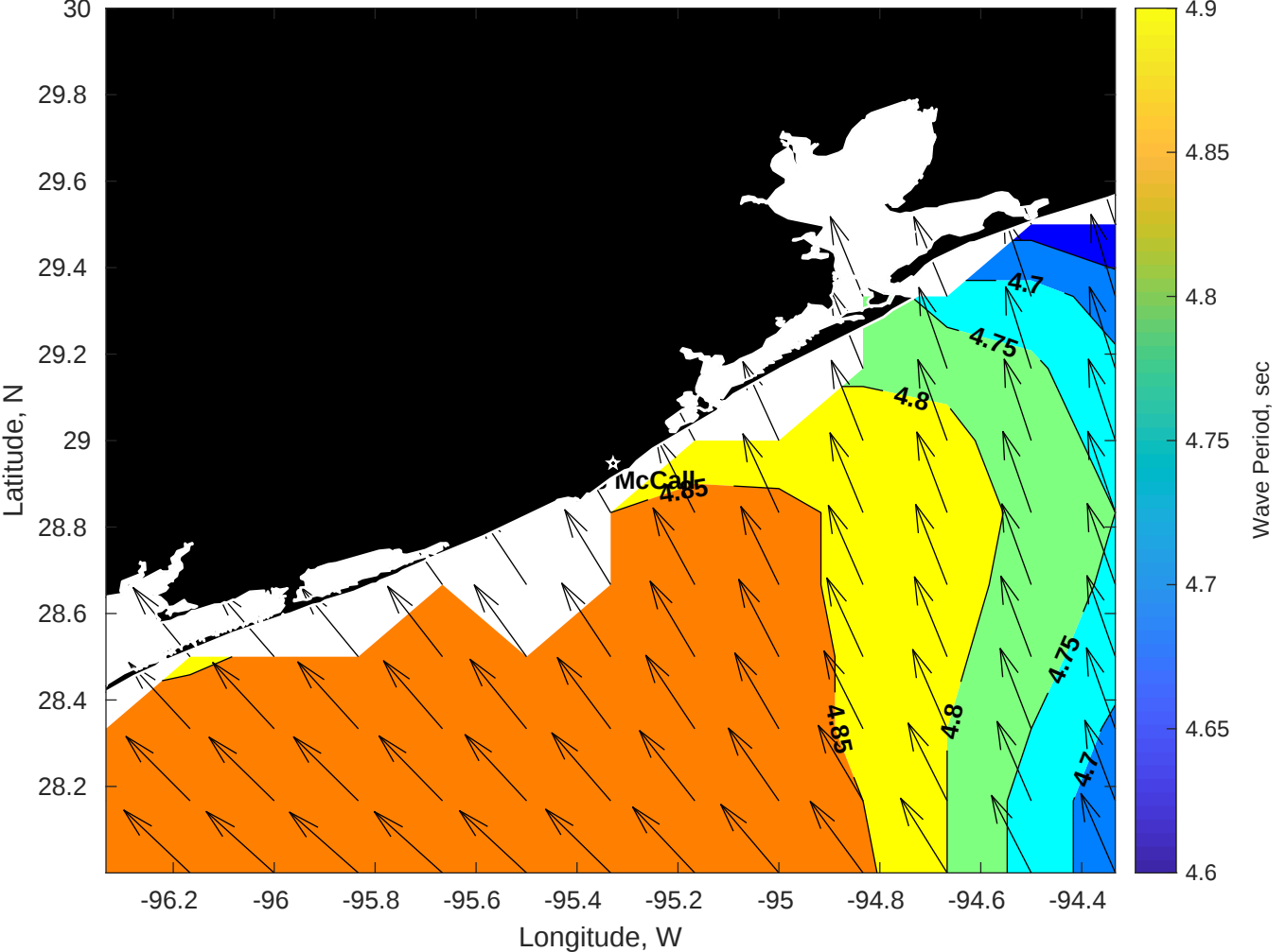
Wave Period (sec) for Brooks McCall at 18-Aug-2025 09:00:00
