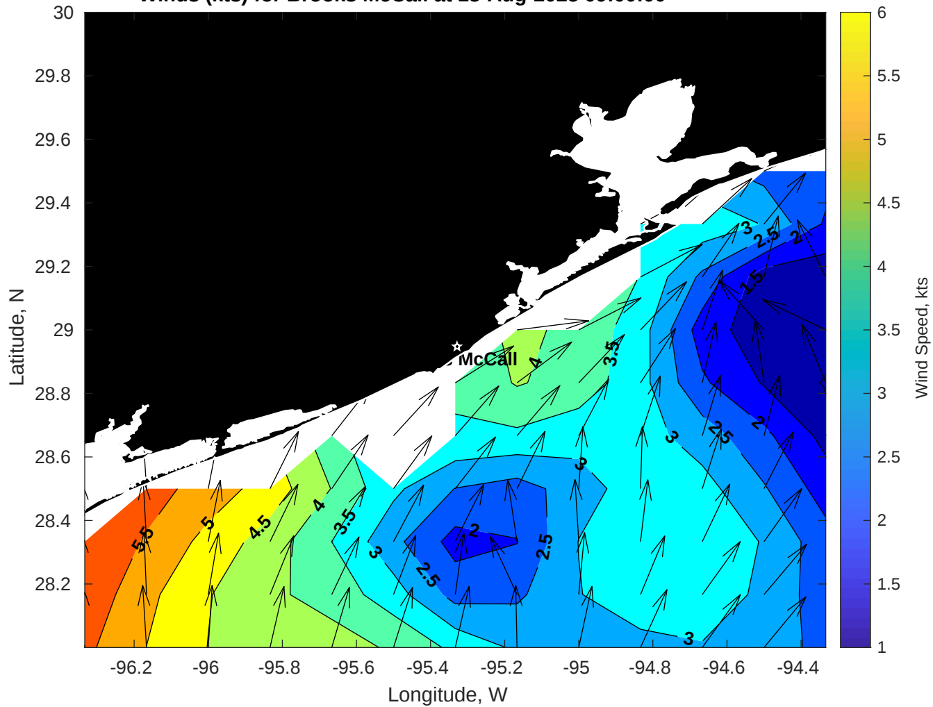
Winds (kts) for Brooks McCall at 18-Aug-2025 09:00:00
