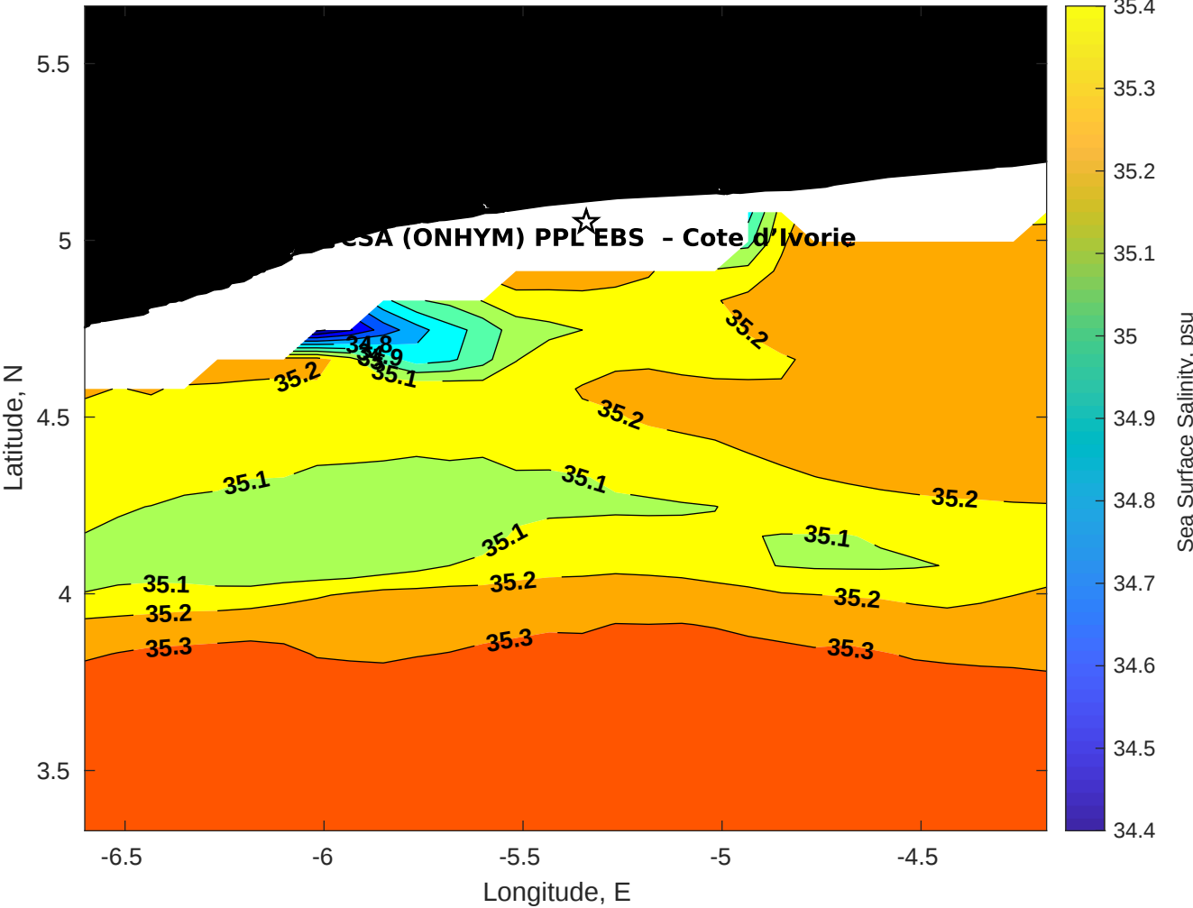
Surface Salinity for CSA (ONHYM) PPL EBS - Cote d'Ivoire at 17-Aug-2025 00:00:00
