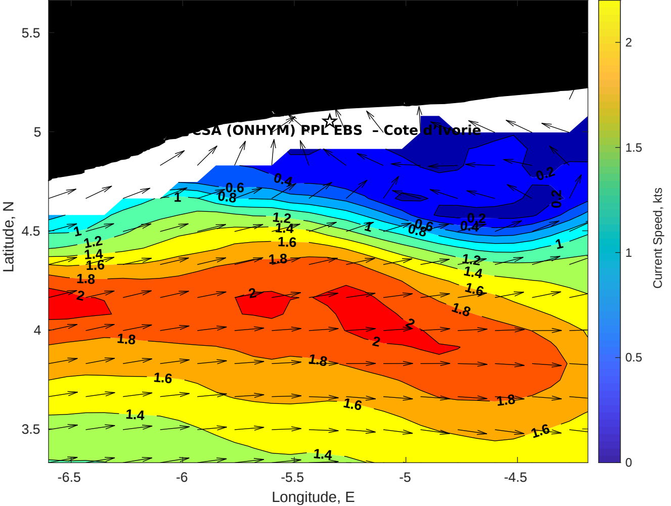
Surface Currents for CSA (ONHYM) PPL EBS - Cote d'Ivoire at 17-Aug-2025 00:00:00
